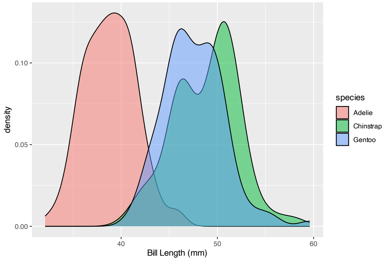
Density Plot of Bill Length
