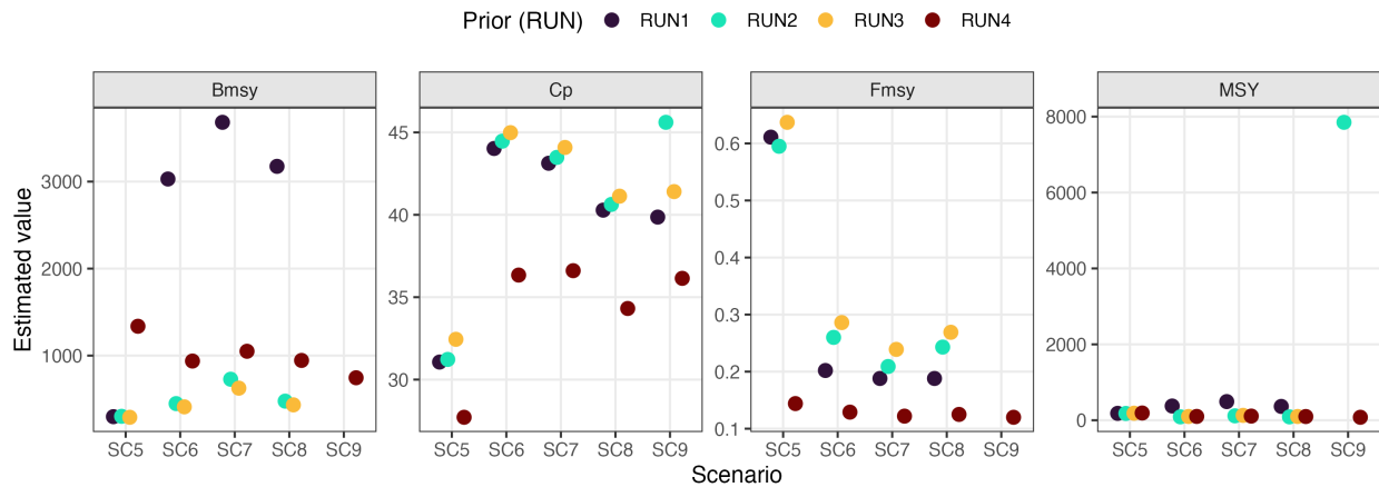
Figure 6: Comparison of stochastic biological reference points (Bmsy, Fmsy, MSY) and current catch (Cp) across SPiCT Scenarios SC5–SC9 and prior configurations (RUN1–RUN4) for Nephrops FU30. Points represent scenario–prior combinations, illustrating the sensitivity of stock productivity and exploitation reference points to alternative data configurations and prior assumptions.
