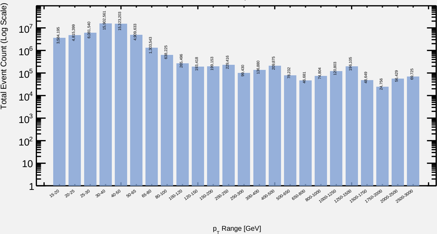
Event Distribution vs p_T (Log Scale Y-Axis)
