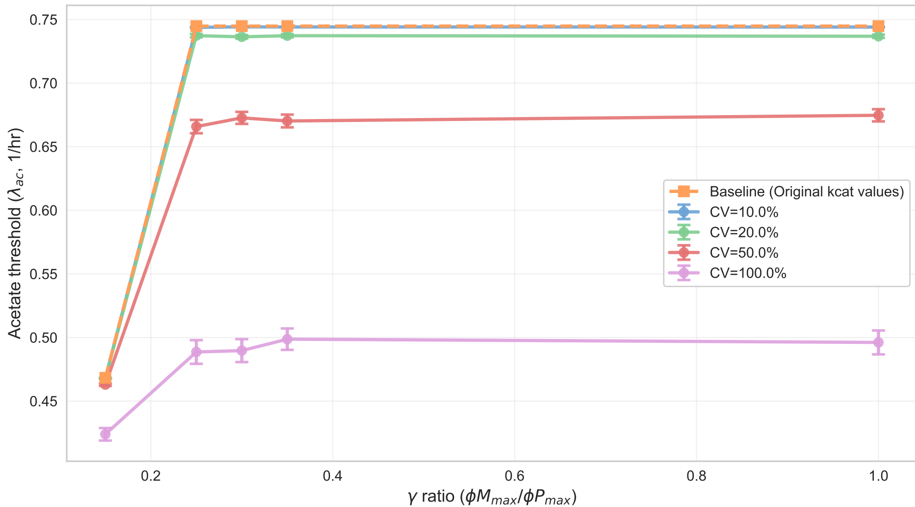
Sensitivity analysis of kcat uncertainty by Monte Carlo sampling
