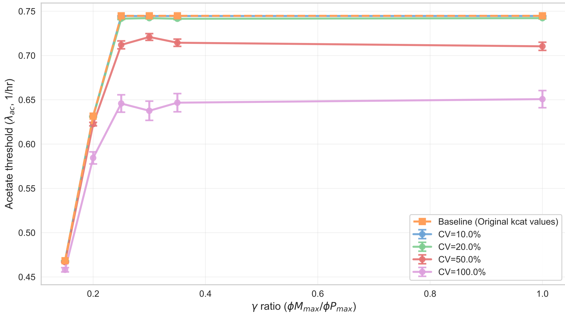
Sensitivity analysis of membrane kcat uncertainty by Monte Carlo sampling
