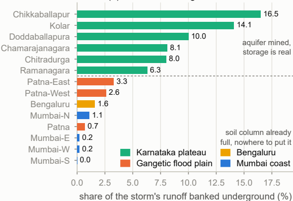
(a) metered recharge, not assumed
