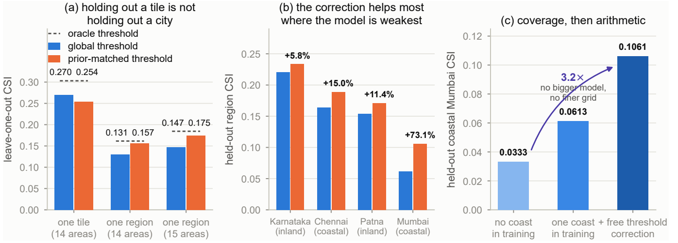
Fig. 6. The three results of Section V. (a) The same model on the same scenes scores 0.270 or 0.147 depending only on whether the held-out area still has siblings in training, so the split and not the model sets the headline. The dashed rule is an oracle threshold chosen while looking at the answer, and the free correction captures most of the distance to it. (b) That correction is worth +73 % on the region the model understands least and almost nothing on the one it understands best. (c) Held-out coastal Mumbai, from having no coast in training, to having one, to having the threshold correction as well.
