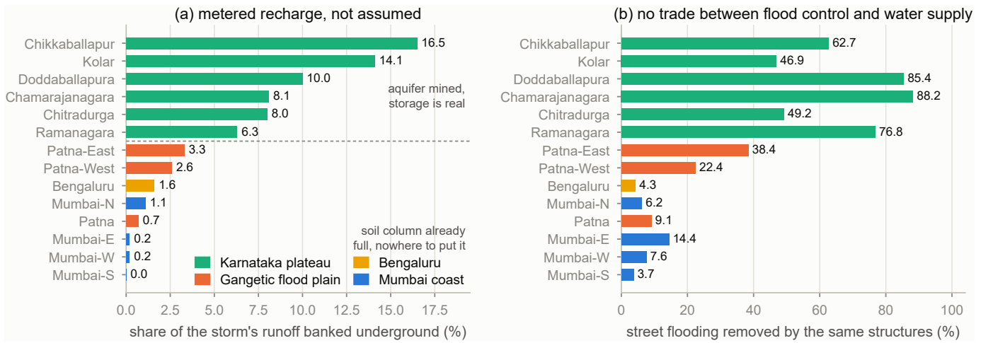
Fig. 11. Recharge measured rather than assumed, across all fourteen built areas. (a) The share of a 100 mm storm's runoff that actually reaches the aquifer, read off the simulation after the structures are built, splits cleanly at the dashed line. The six Karnataka plateau towns bank 6.3 to 16.5 % because their aquifer is mined and the soil column has room, while the flood plain and the coast manage 0.7 to 3.3 % because their soil is already close to full. (b) The same structures remove 46.9 to 88.2 % of street flooding in those towns, so where recharge works it is not a trade against flood control but the same intervention.
