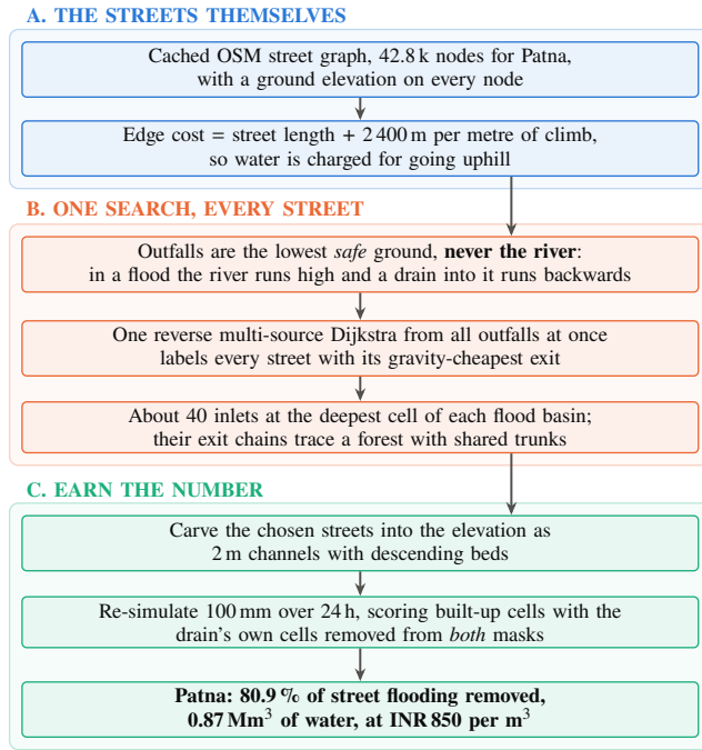
Fig. 8. How the drain network is designed, and how its number is earned. The whole plan falls out of one graph search over the real streets. The reduction it claims is not estimated from pipe capacity but measured by running the design storm again over the carved ground, and taking the drain's own cells out of both the before and the after mask is what stops the planner from being credited for moving water onto a drain.
