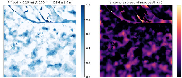
Fig. 5. Why routing water downhill cannot place it. Ten elevation models drawn from FABDEM’s own error class, each simulated at 100 mm. Left, the share of the ten runs that flood each cell, where white means almost none of them and dark blue means almost all. Right, the spread in predicted depth. Total flooded area is stable at 10.79 \pm 0.35 \text{ km}^2 , but only 5 % of Patna’s flooded area is agreed on by nine runs in ten, so the size of the flood is firm while its position is not.
