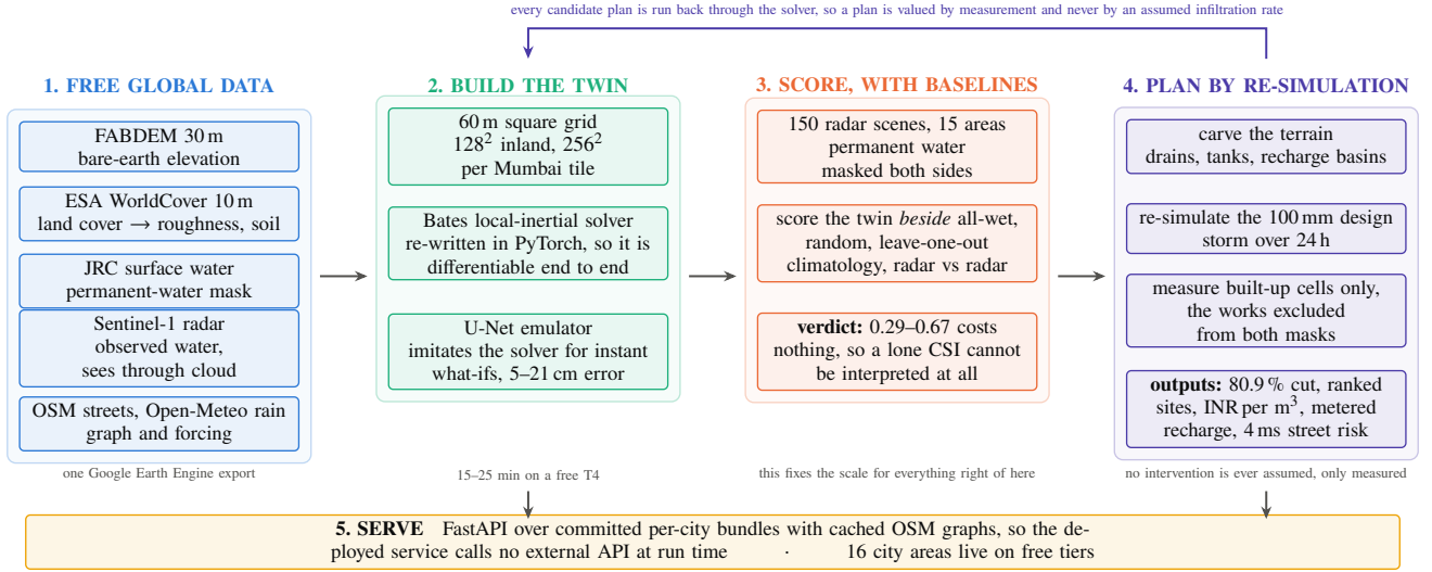
Fig. 2. The whole process, read left to right. Four free global datasets become a differentiable flood model of any city window in 15 to 25 minutes on a free T4 GPU, that model is scored only ever beside baselines that cost nothing, and every proposed public work is valued by carving it into the ground and running the storm again. The loop drawn above the diagram is why planning survives the location uncertainty of Section IV, because a plan is measured rather than assumed.
