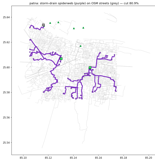
Fig. 9. The design of Fig. 8 on the ground in Patna. Grey is the OpenStreetMap street network, purple is the chosen drain, drawn thicker where more basins share a trunk, the small purple dots are inlets, the green squares are the safe lowland outfalls the search chose, and the green triangles are river outfalls it was forbidden to use. No part of this network is drawn by hand.
