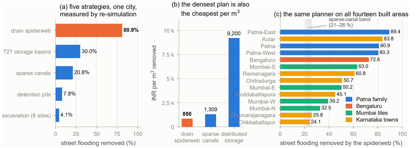
Fig. 10. Every planning result, all of it measured by re-simulation. (a) Five strategies on one city, where the dense network beats the best sparse alternative by a factor of four. (b) It is also the cheapest per cubic metre of water actually removed, because trunks shared between basins spread their length over many of them. (c) The same planner, unchanged, on all fourteen built areas. The grey band marks what the sparse plans achieve, and only two areas fail to clear it.
