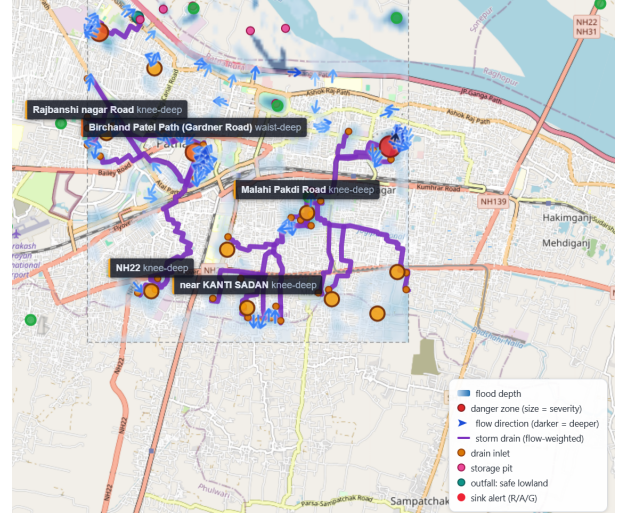
Fig. 1. The live system for Patna at a 100 mm design storm. Blue is predicted depth, arrows show flow, purple lines are the drain network the planner designed on the real street graph, and labels name real streets with a depth in words rather than a number.
