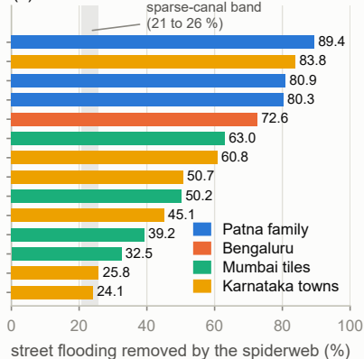
(c) drain network in all fourteen built areas
