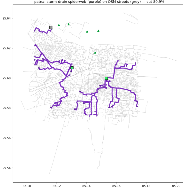
Figure 2: The planned storm-drain spiderweb for Patna (purple; line width \propto accumulated flow) traces real OSM streets (grey) from 40 flood-basin inlets to detention pits and safe low-ground outfalls. Measured cut: 80.9% of street flooding at 100 mm.
