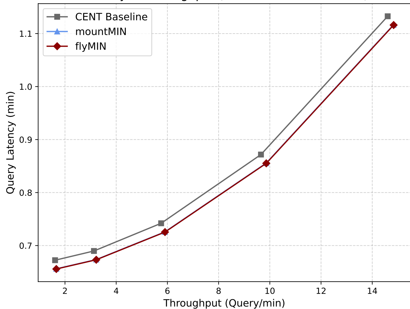
Latency vs Throughput (Llama2-70B, 32 devices)
