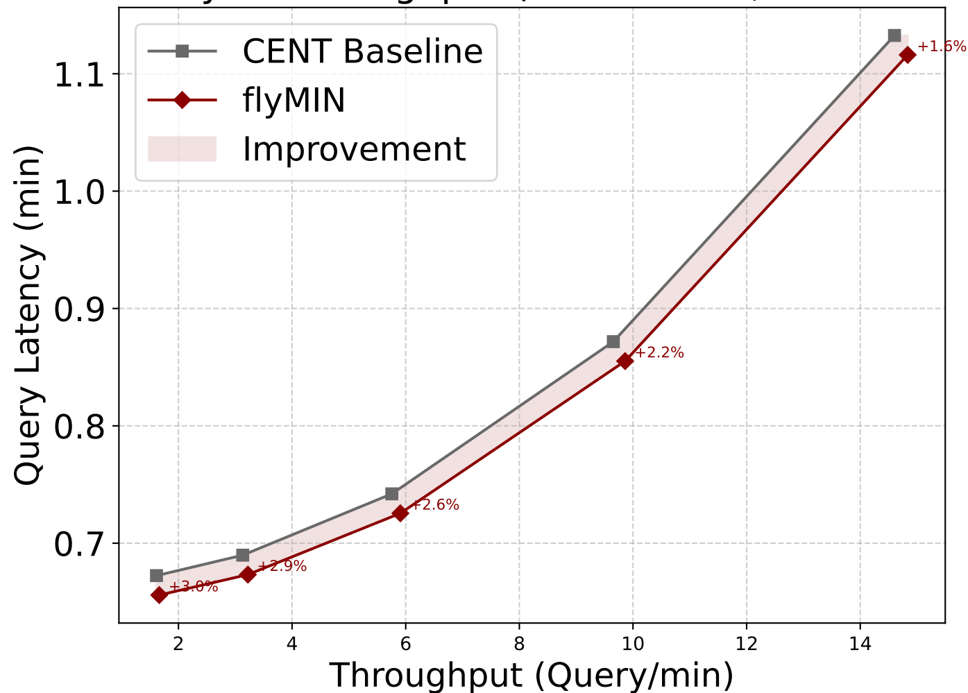
Latency vs Throughput (Llama2-70B, 32 devices)
