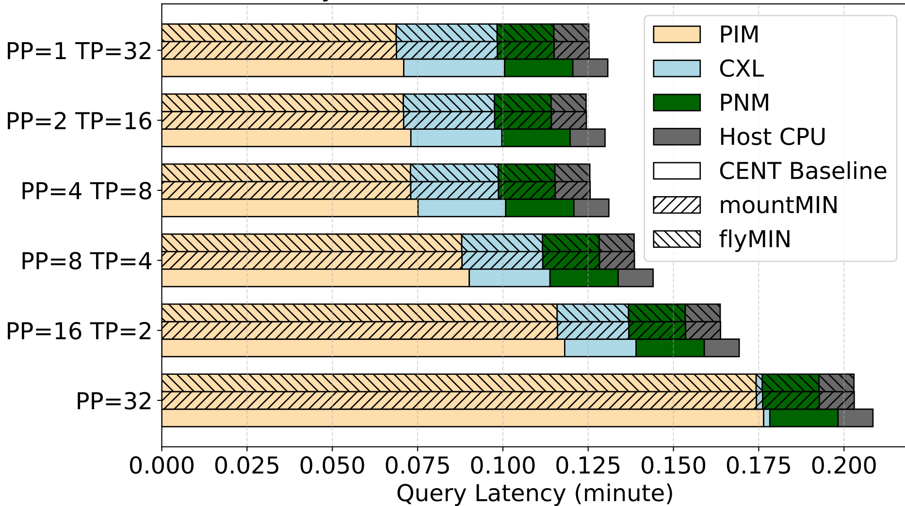
Latency Breakdown: Llama2-7B on 32 Devices
