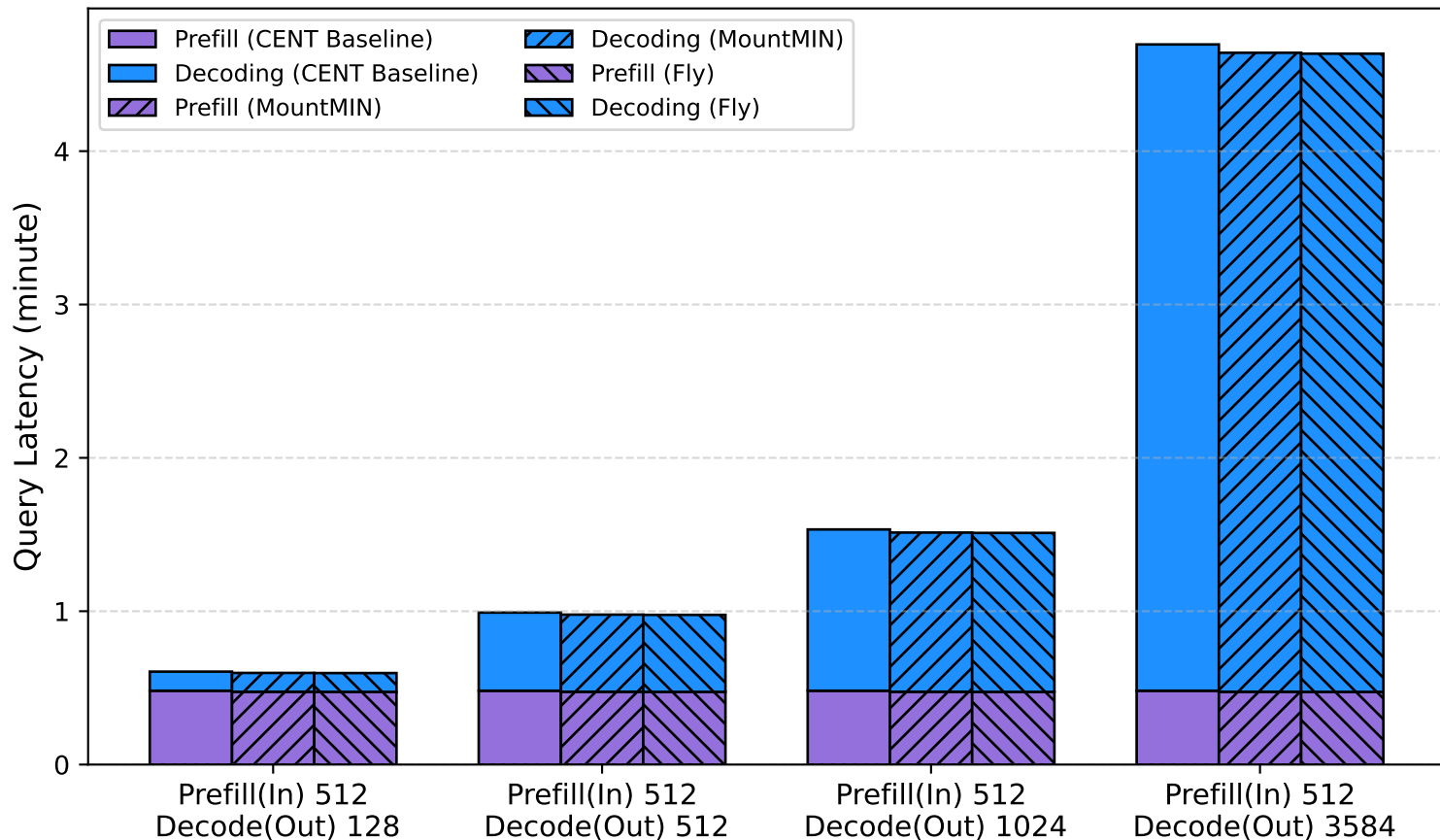
14d: Llama2-70B - 32 Devices (Comparison)
