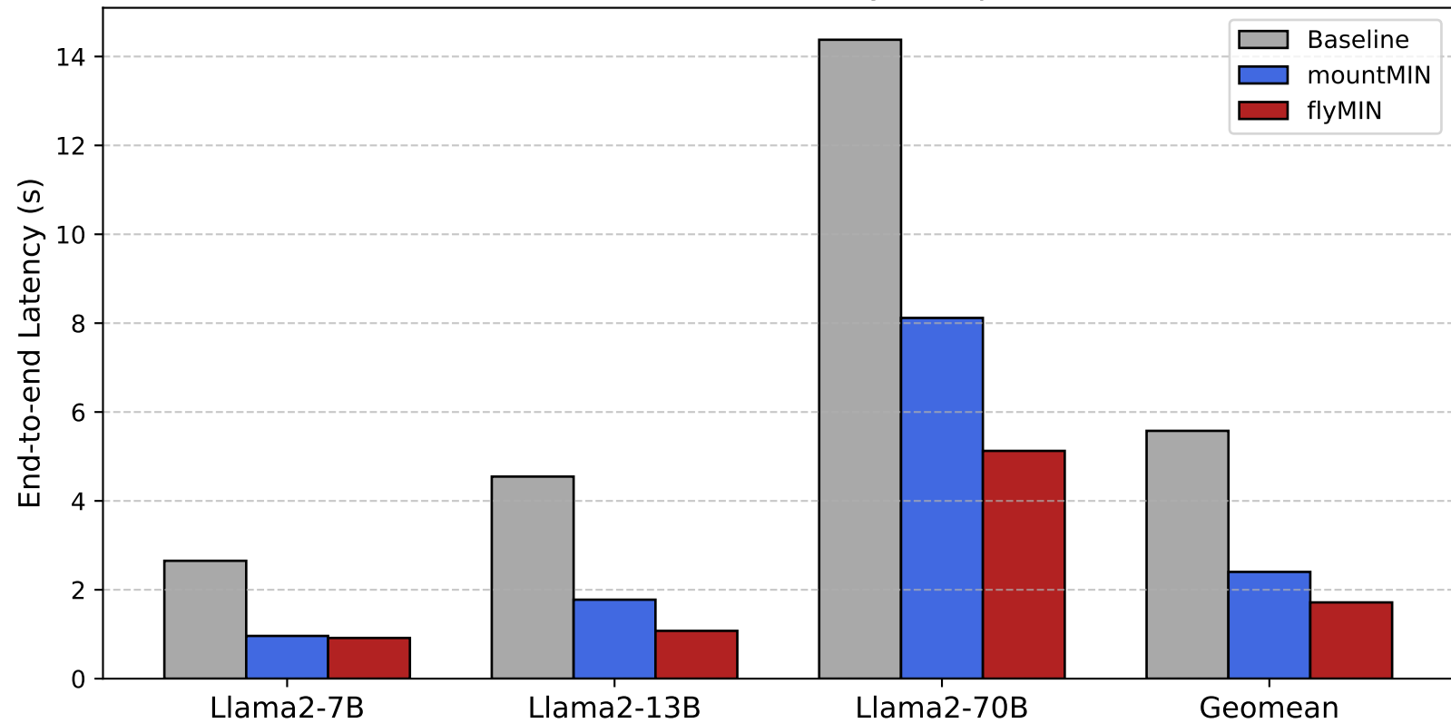
ROPE End-to-end Latency Comparison
