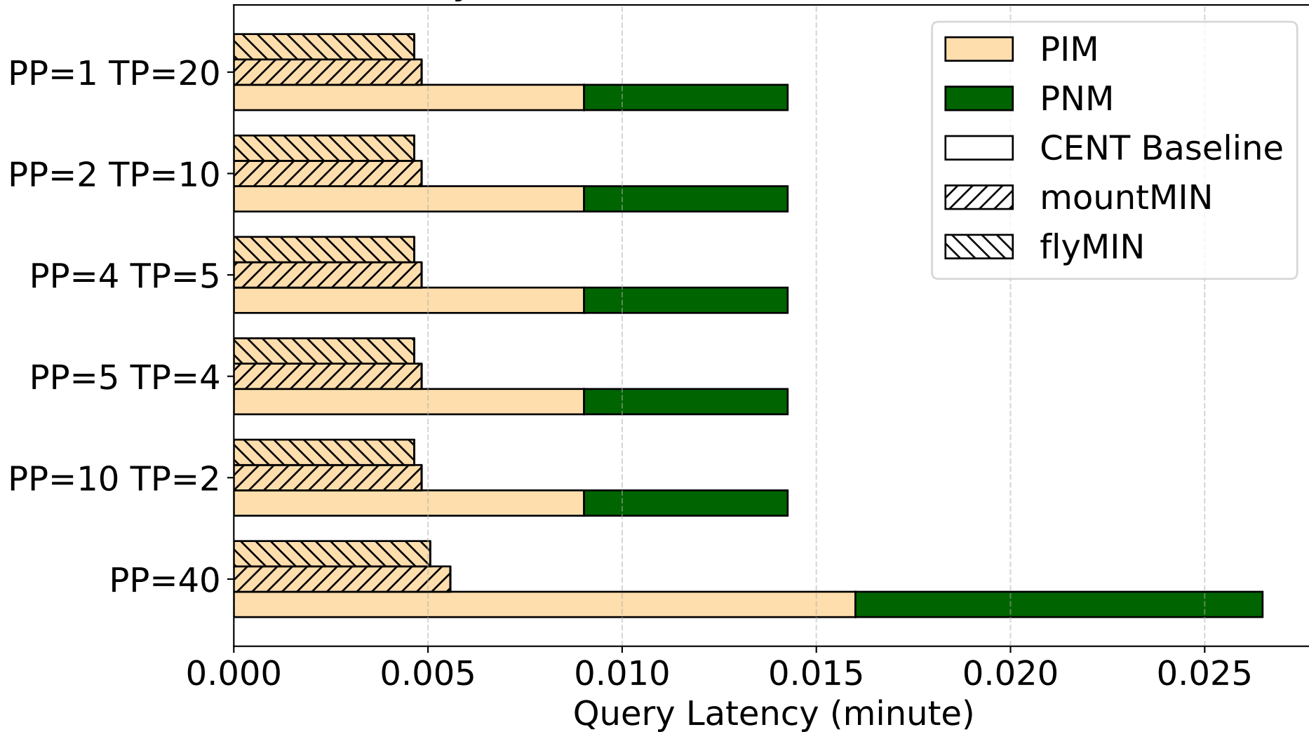
Latency Breakdown: Llama2-13B on 20 Devices
