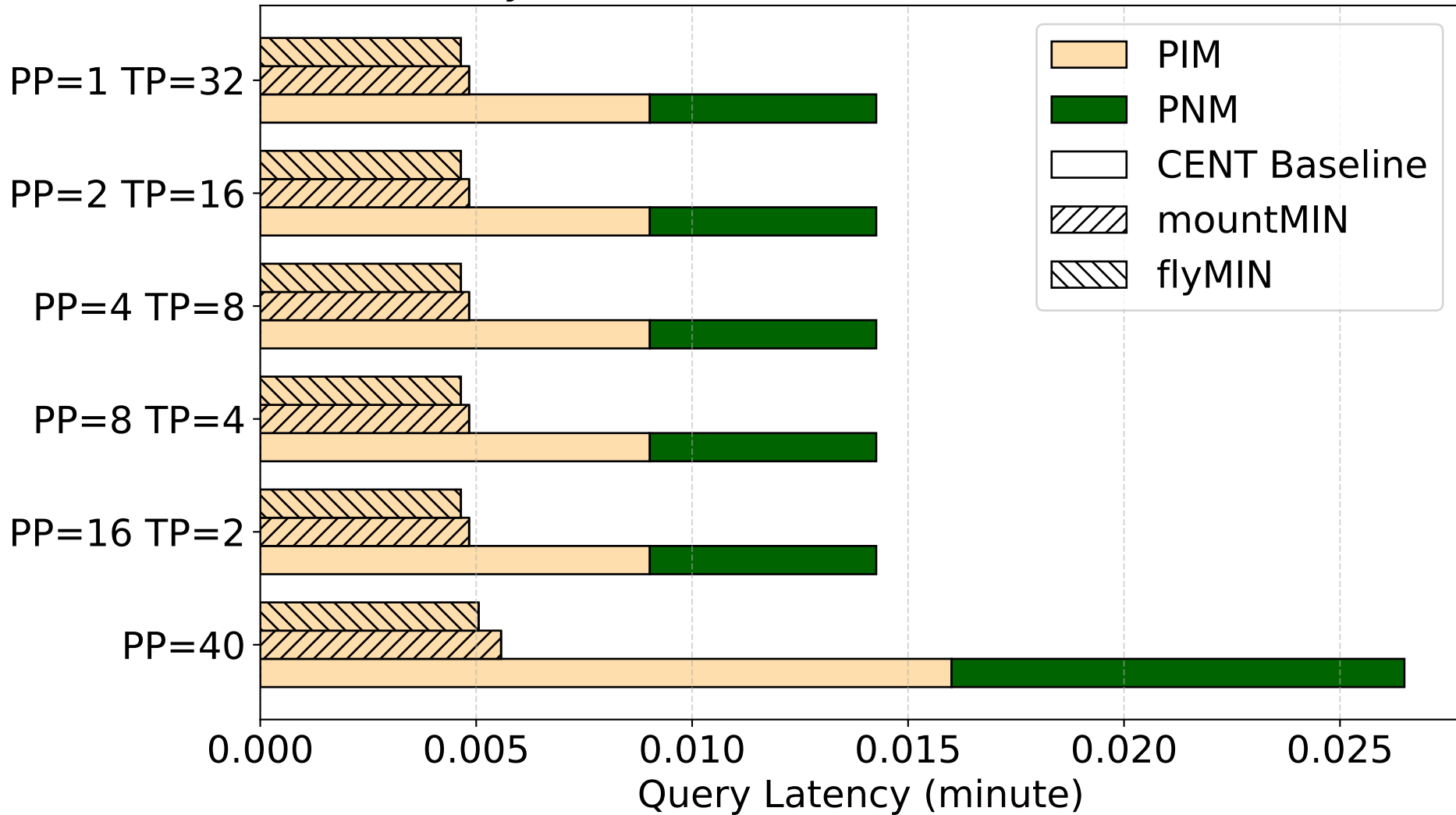
Latency Breakdown: Llama2-13B on 32 Devices
