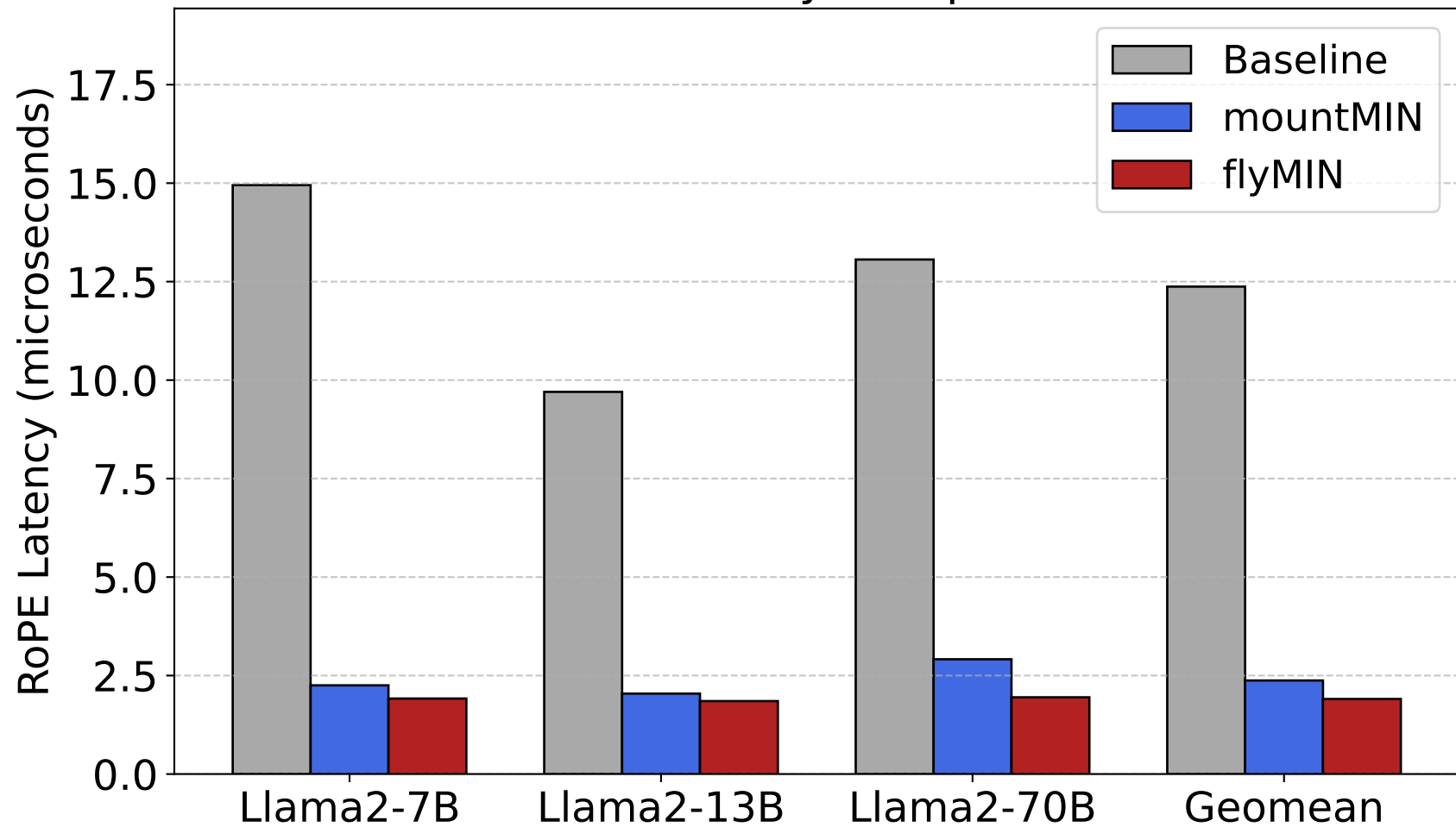
ROPE Latency Comparision
