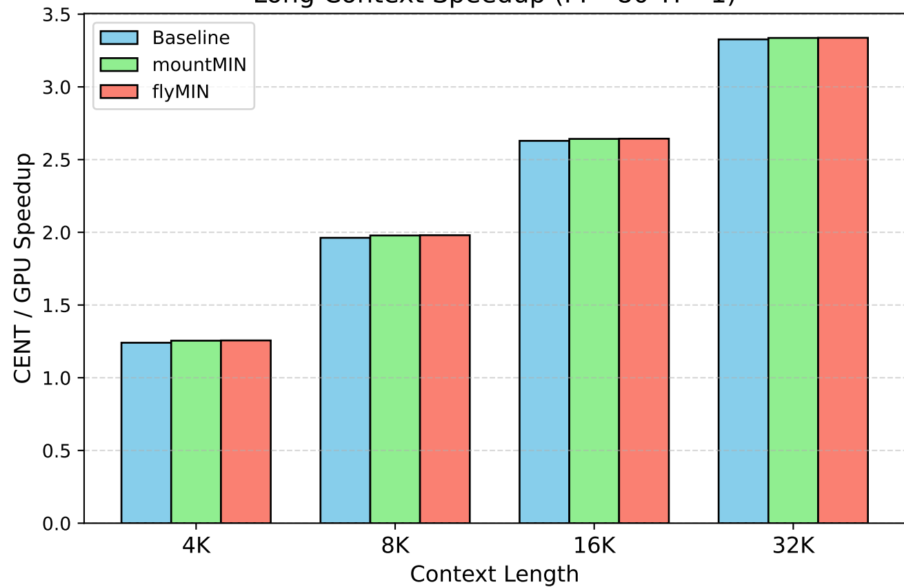
Long Context Speedup (PP=80 TP=1)
