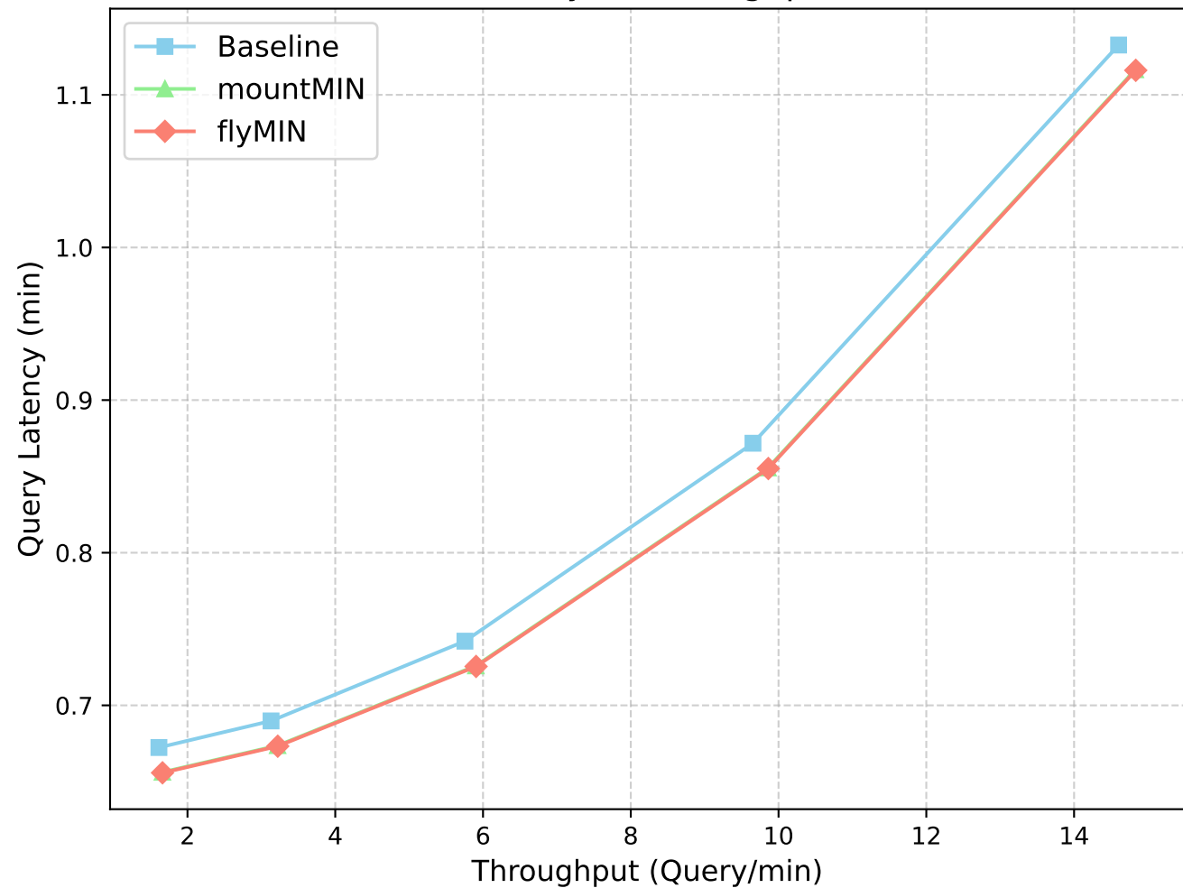
Latency vs Throughput
