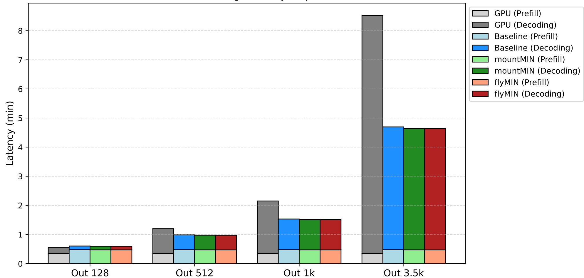
Prefill + Decoding Latency (Input 512)
