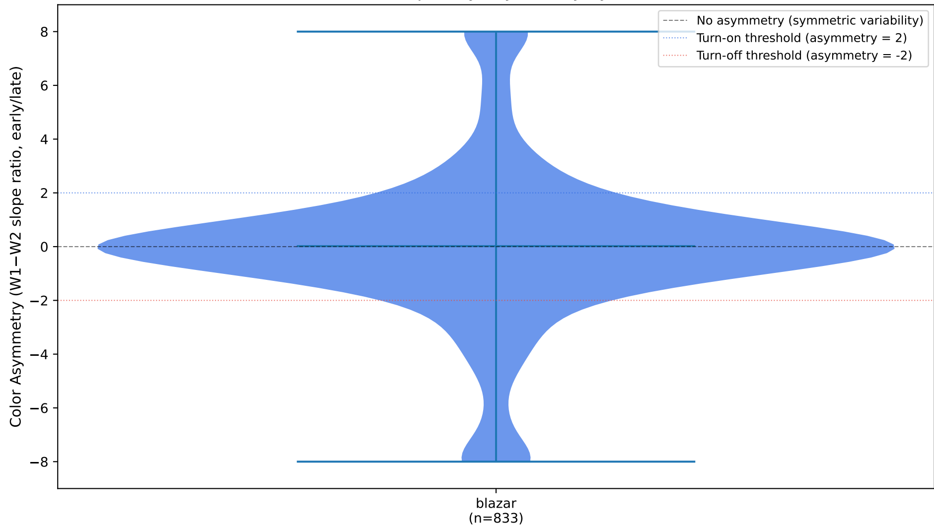
W1–W2 Color Trajectory Asymmetry by Source Class
