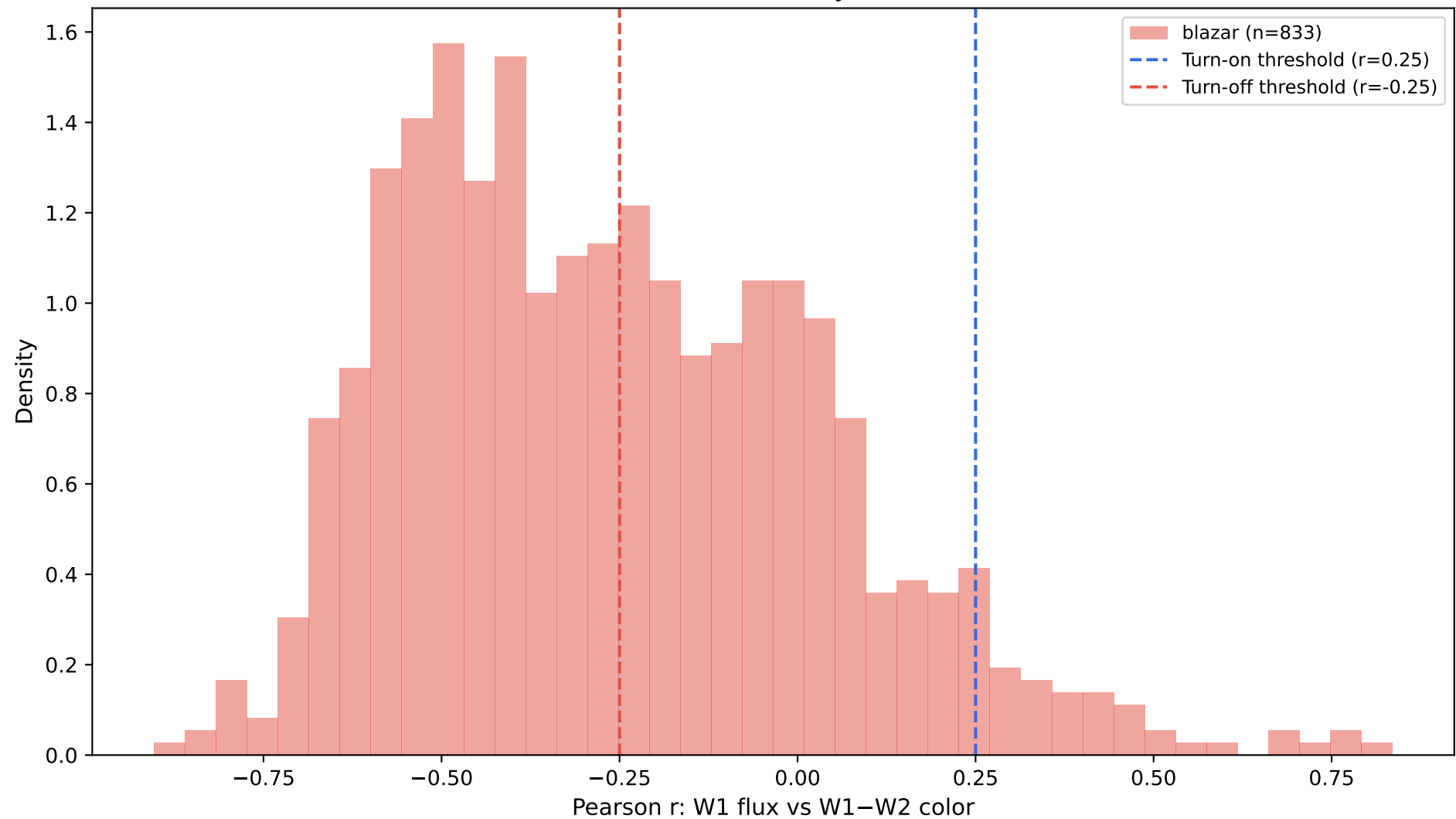
Flux-Color Correlation by Source Class
