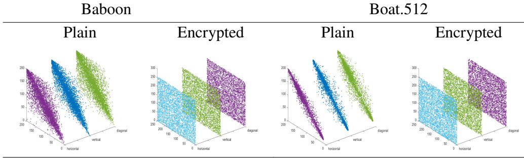
Figure 2: Baboon, Boat.512 images: plain image and its corresponding cipher image correlation plots.
