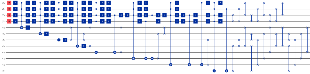
Figure 4: Dual Baker quantum circuit.
