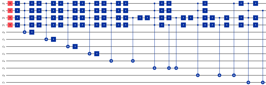
Figure 3: GNEQR quantum circuit.
