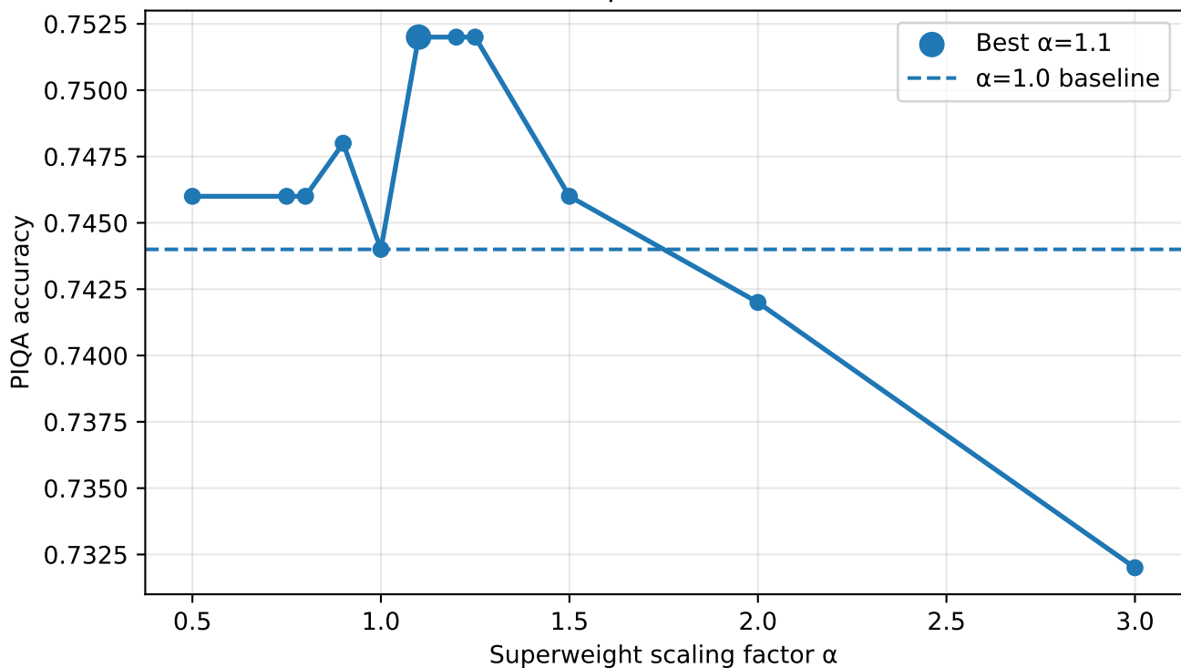
Effect of Superweight Scaling on PIQA Accuracy OLMo-1B, Super W8 Quantization
