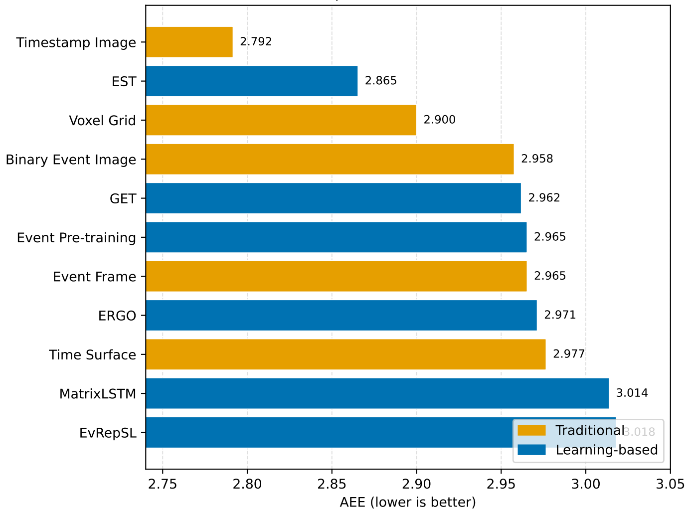
MVSEC Optical Flow: Unified Protocol
