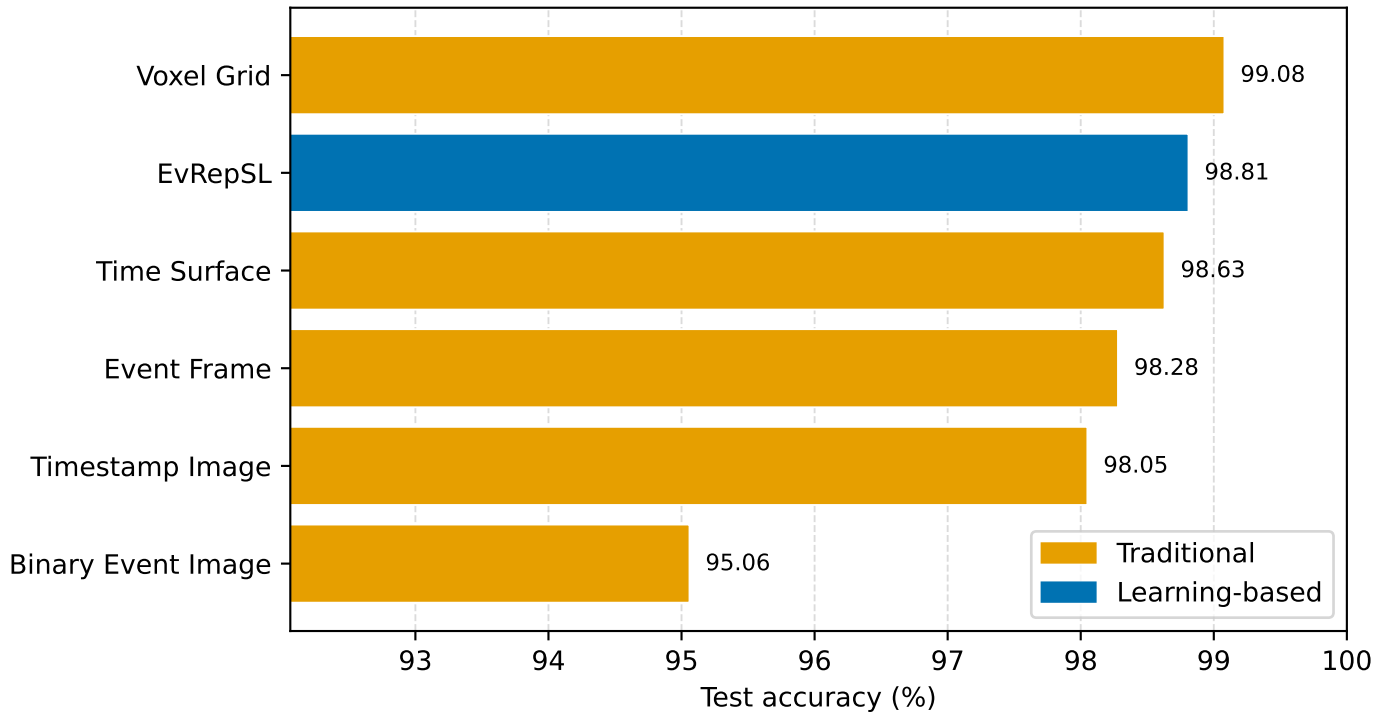
N-MNIST Classification
