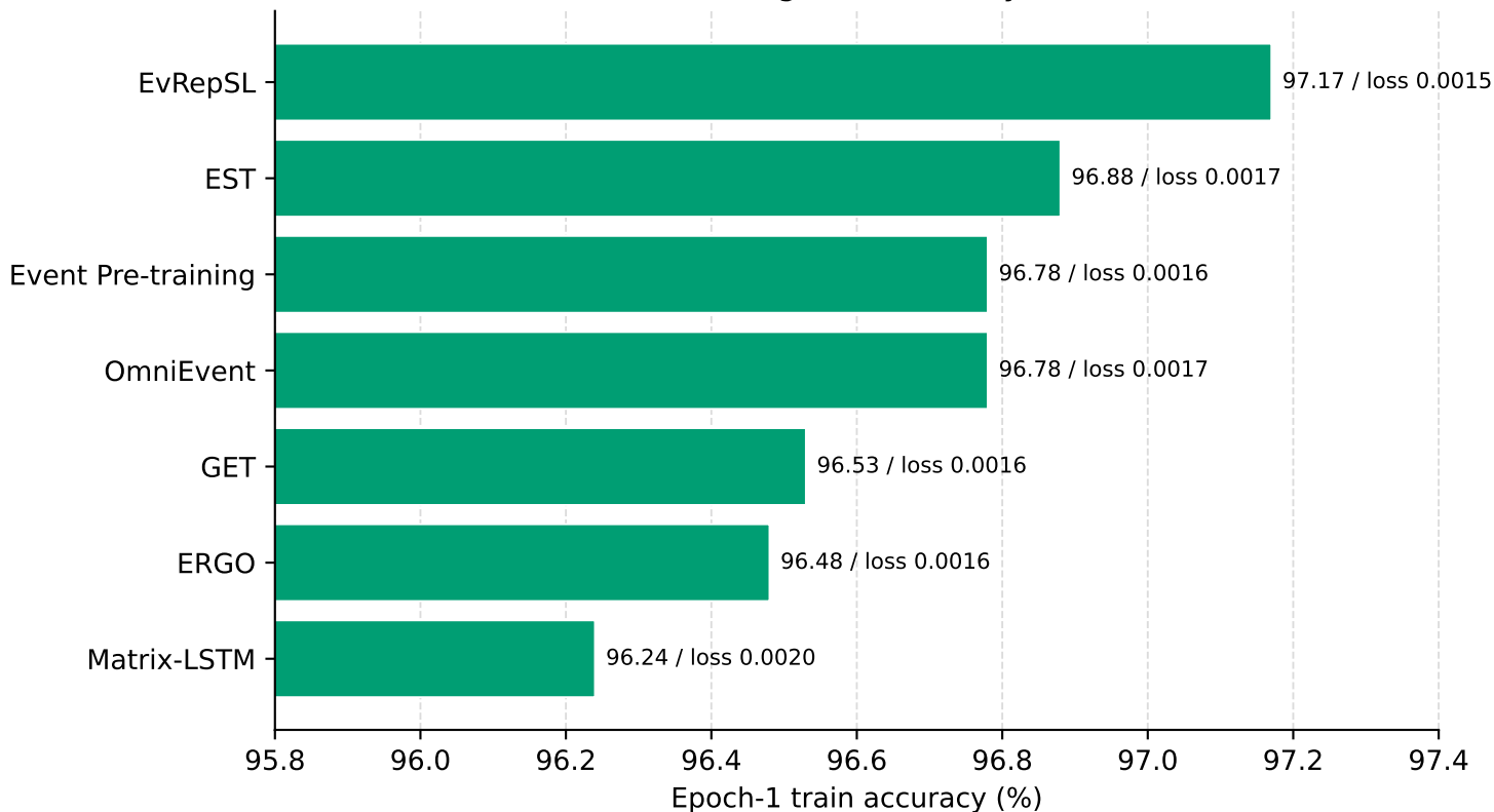
N-MNIST Learning-based Sanity-scale Runs
