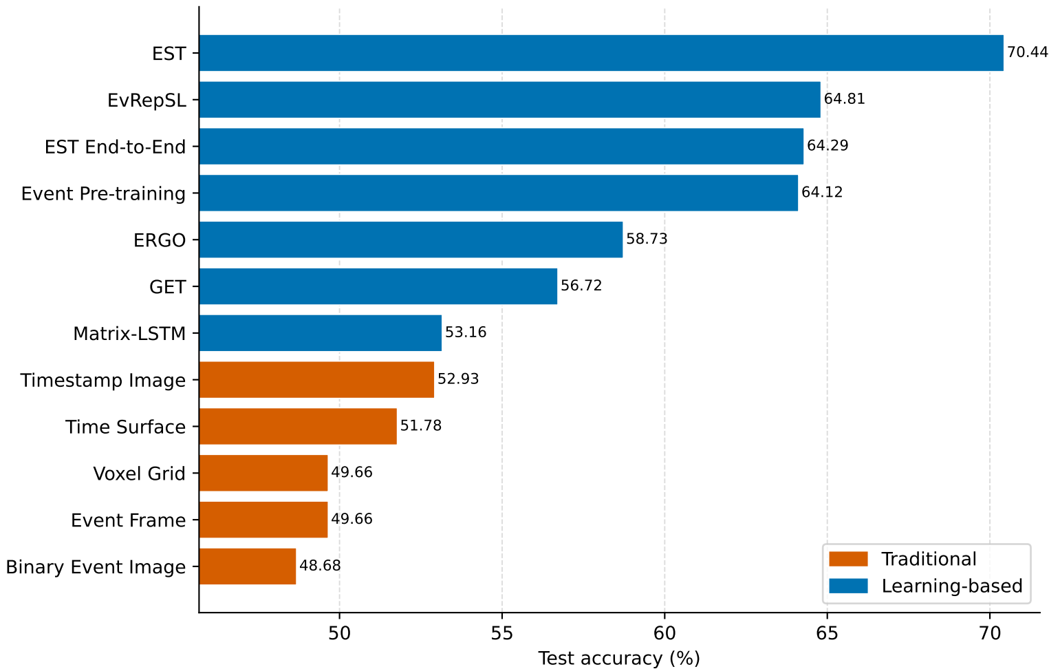
N-Caltech101 Classification (Latest)
