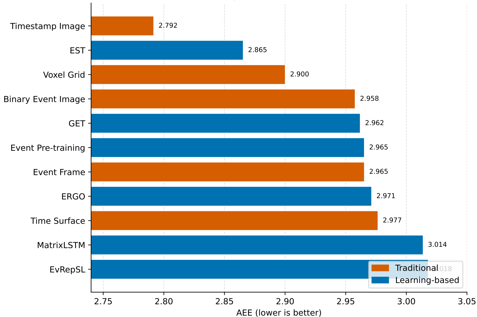
MVSEC Optical Flow: Unified Protocol
