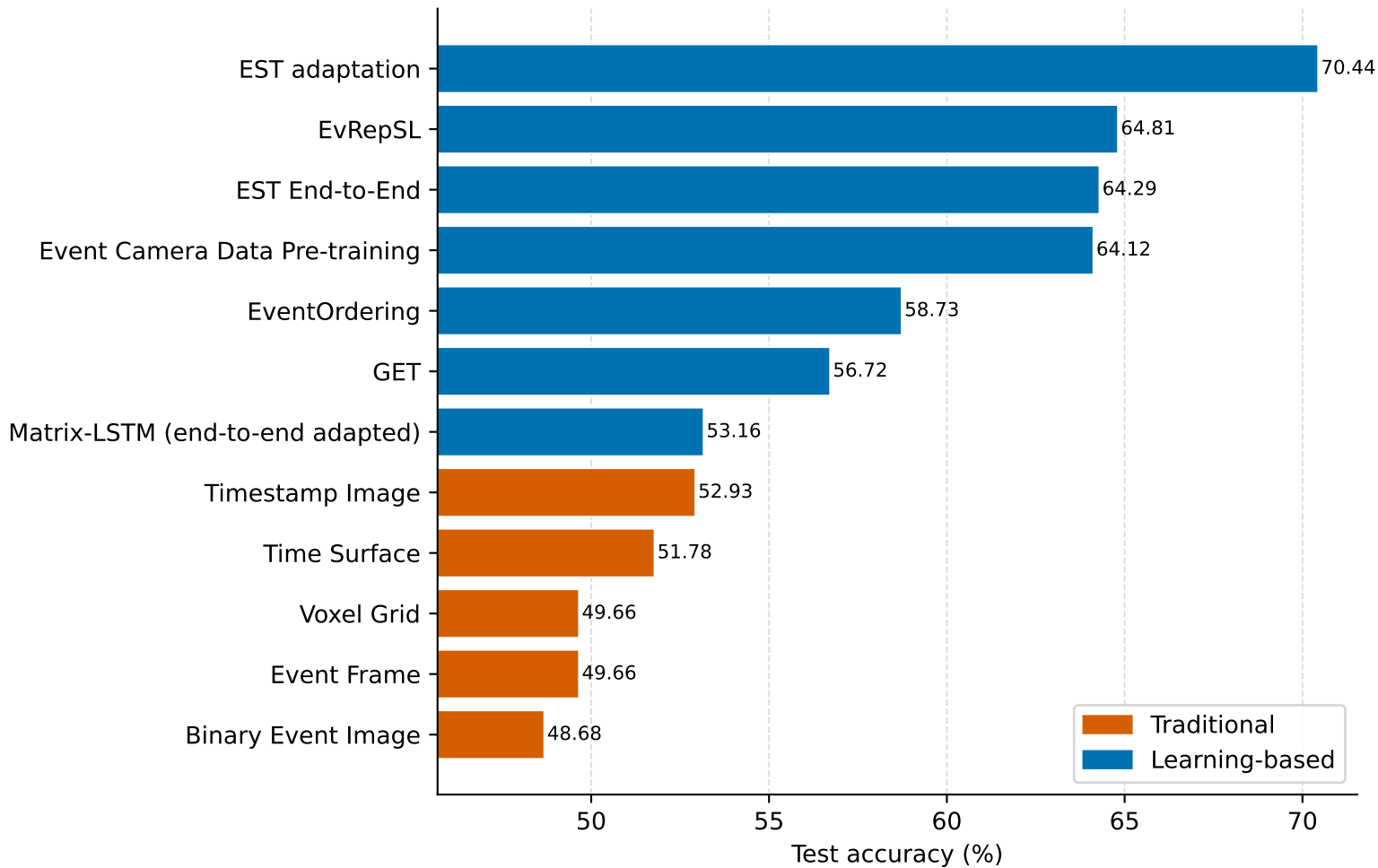
N-Caltech101 Classification
