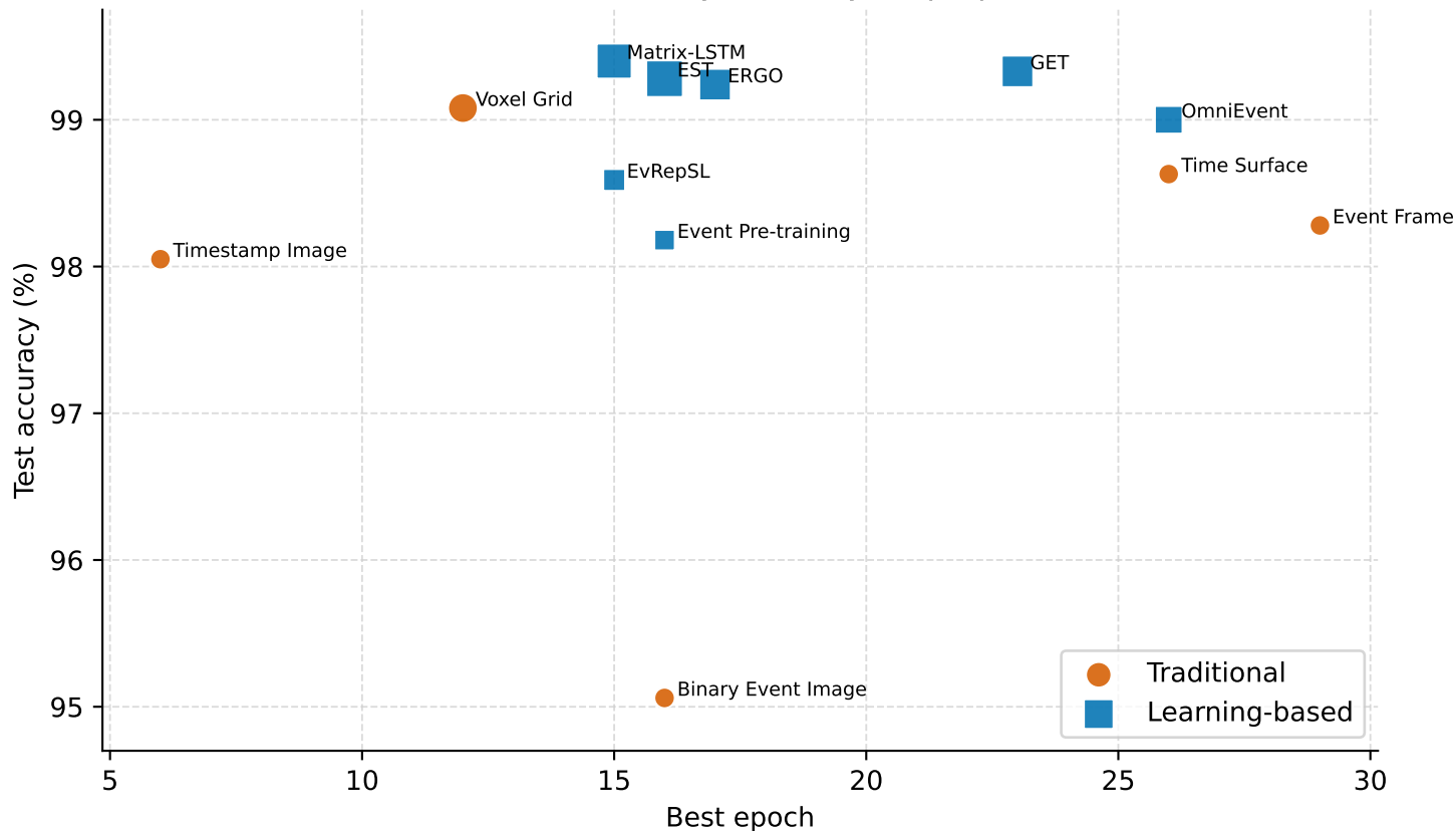
N-MNIST Accuracy vs. Early-stop Epoch
