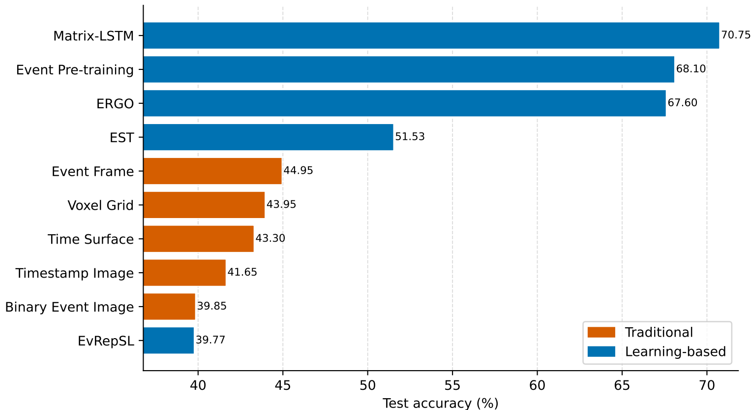
CIFAR10-DVS Classification (Latest)
