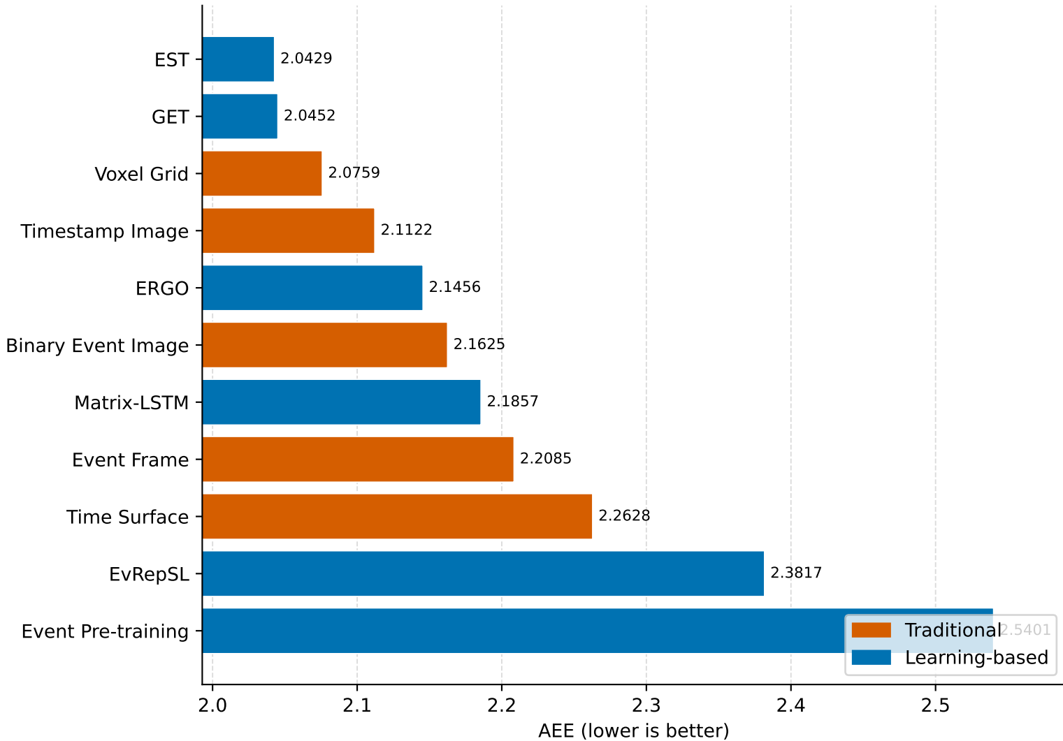
MVSEC Optical Flow (Unified Protocol)
