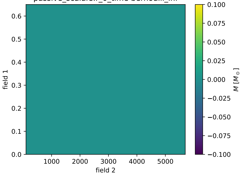
passive_scalars.r_0_time bernoulli_inf
