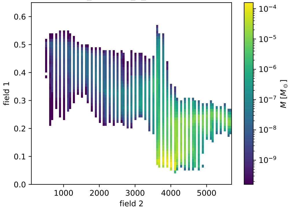
passive_scalars.r_0_time geodesic
