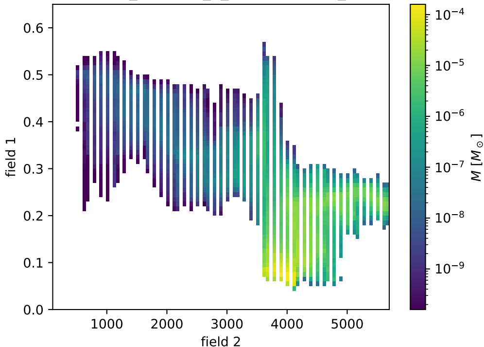
passive_scalars.r_0_time geodesic_out
