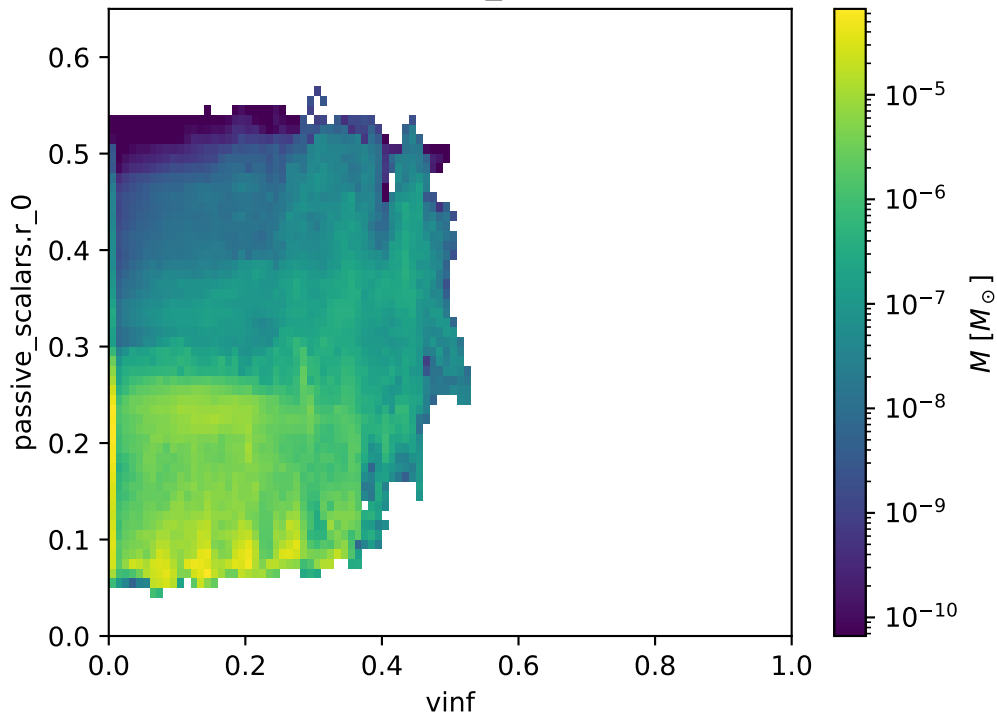
bernoulli_out
