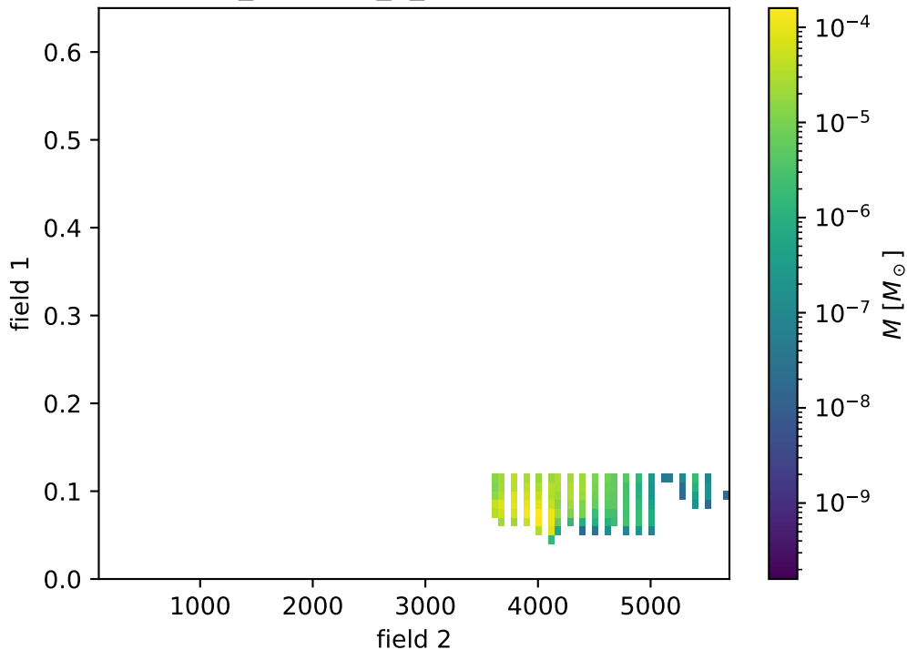
passive_scalars.r_0_time bernoulli tidal
