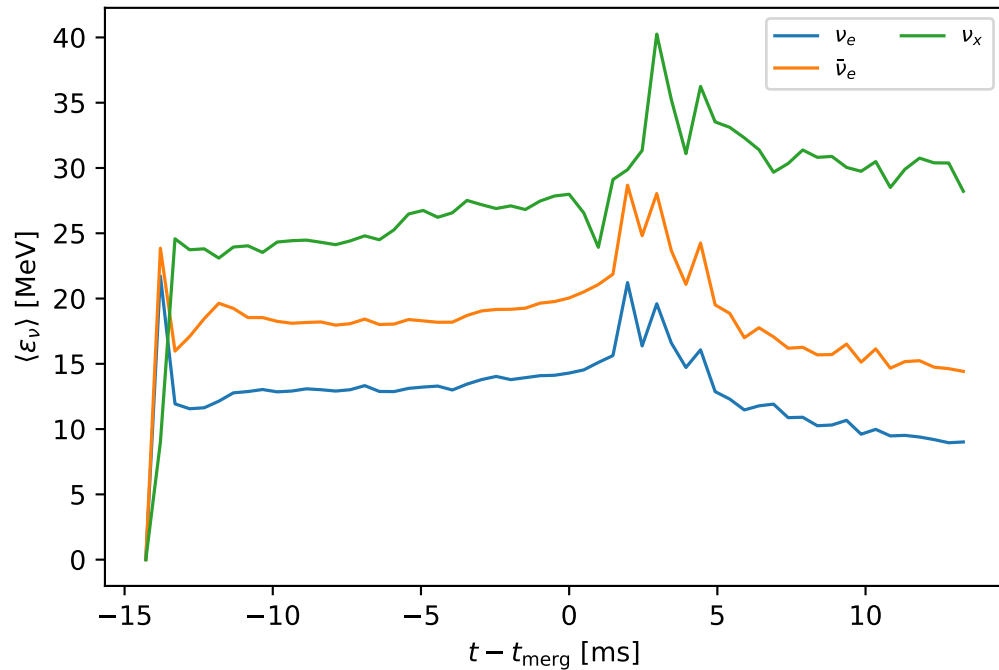
Mean neutrino energy
