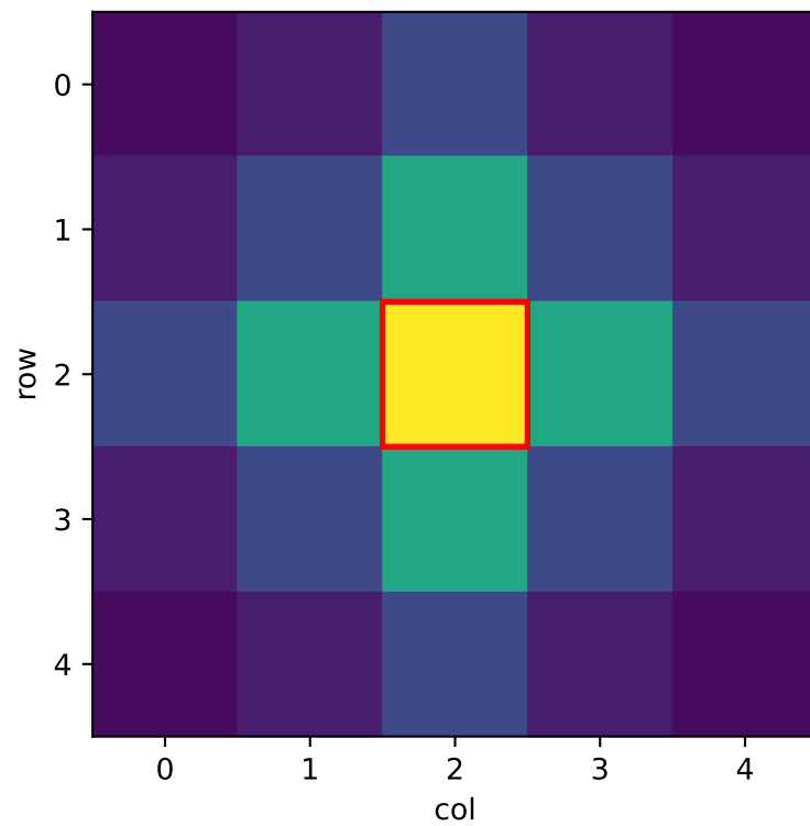
\alpha = 0.6, \lambda = 1.0
