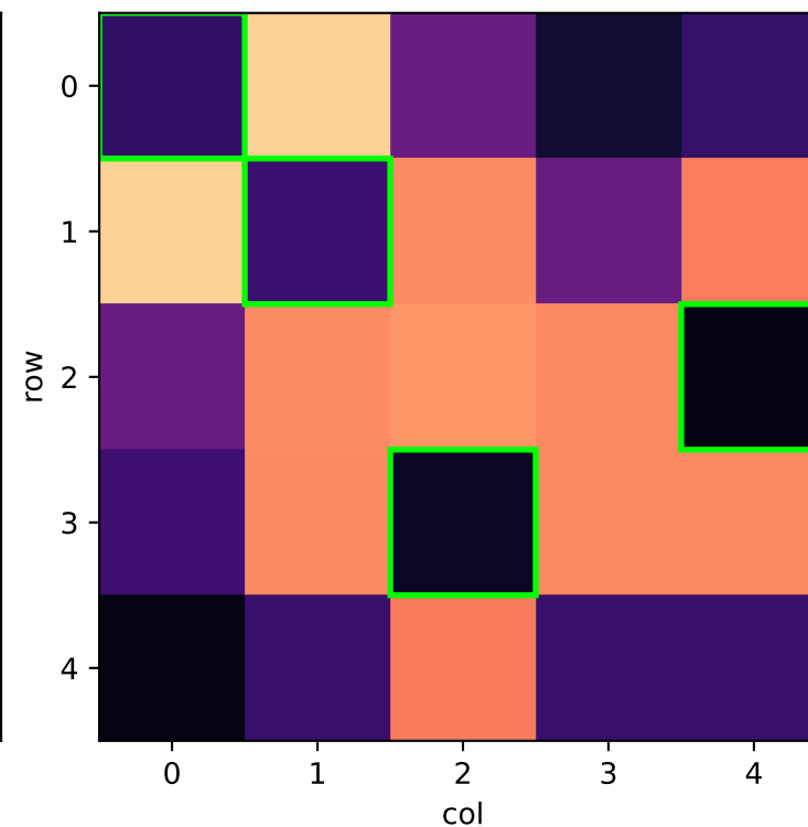
\alpha = 0.8, \lambda = 5.0
