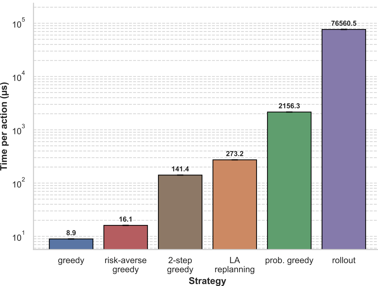
Speed vs Greedy: Absolute time and relative slowdown
