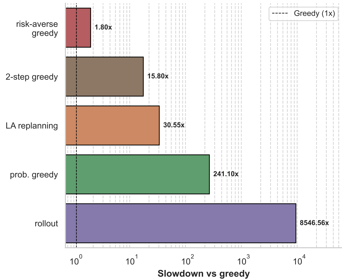
Speed vs Greedy: Absolute time and relative slowdown
