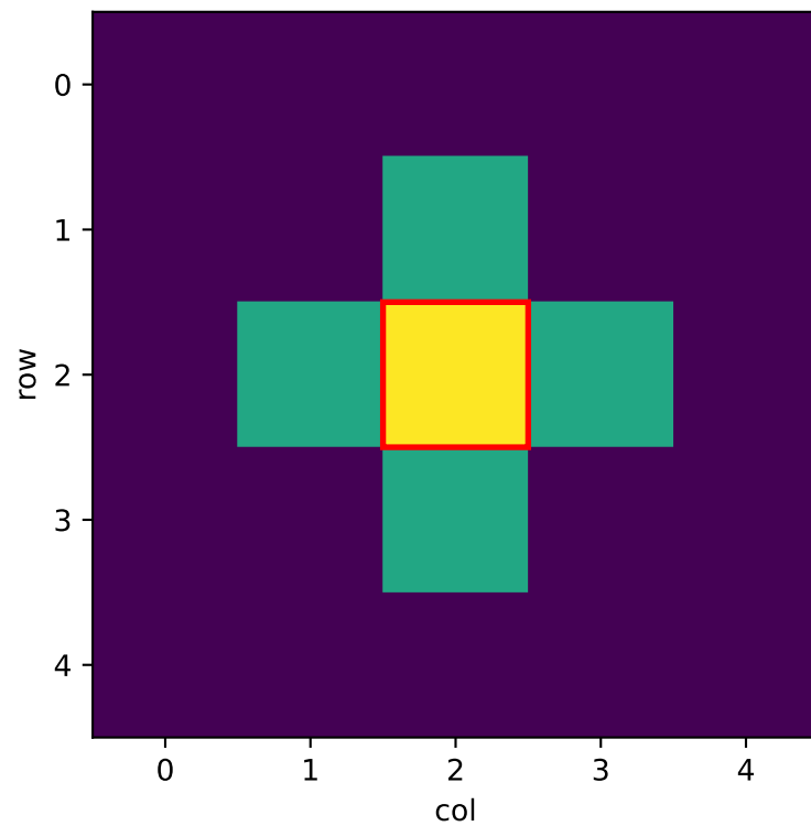
\alpha = 0.6, \lambda = 0.0001
