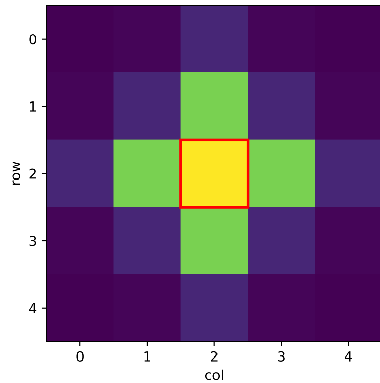
\alpha = 0.8, \lambda = 0.5
