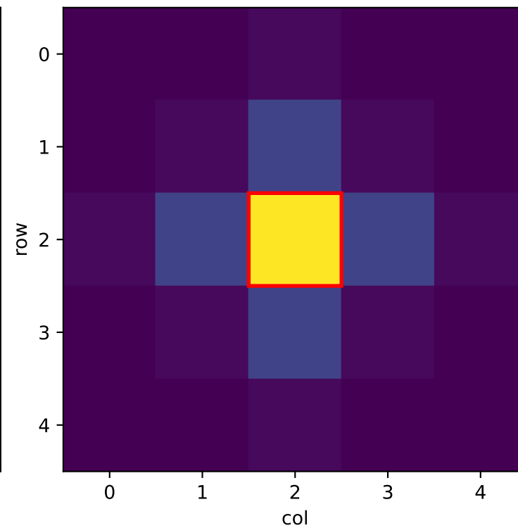
\alpha = 0.2, \lambda = 0.5
