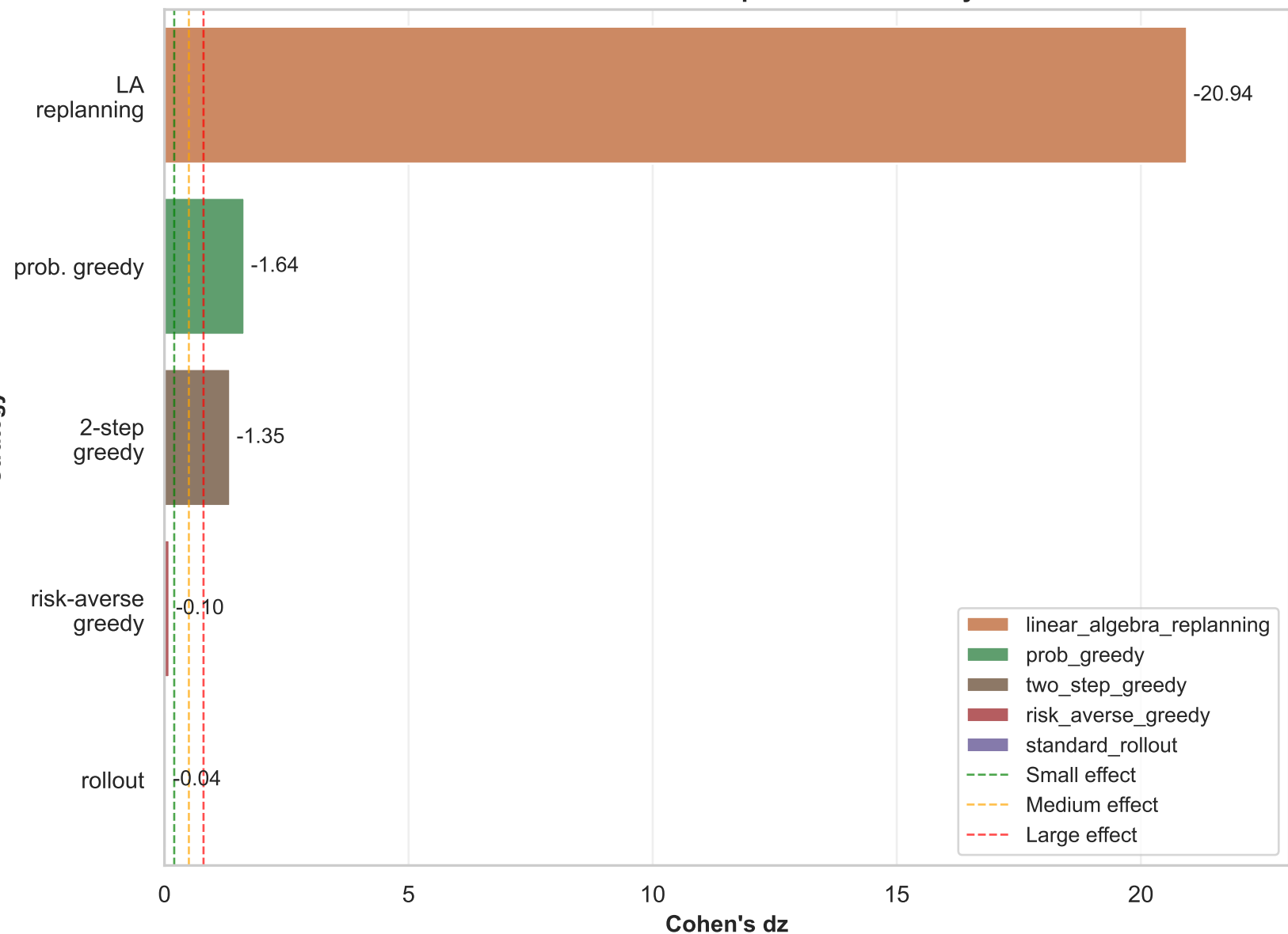
Cohen's dz for Solve Rate Comparisons vs Greedy Baseline
