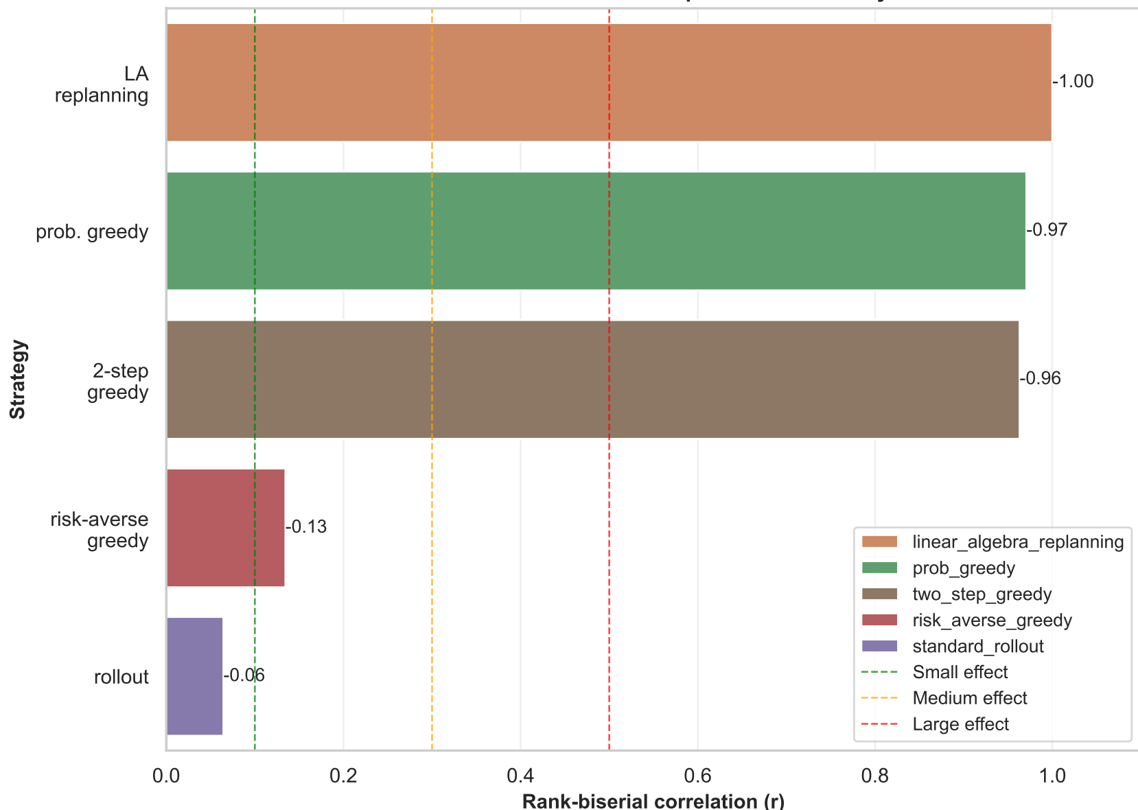
Rank-Biserial r for Solve Rate Comparisons vs Greedy Baseline
