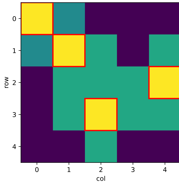
\alpha = 0.6, \lambda = 1.0
