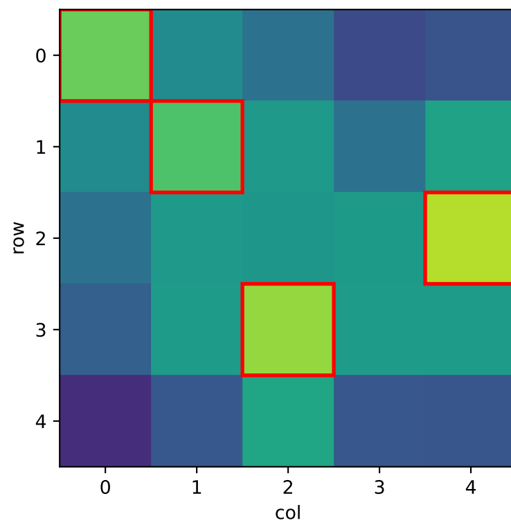
\alpha = 0.6, \lambda = 1.0
