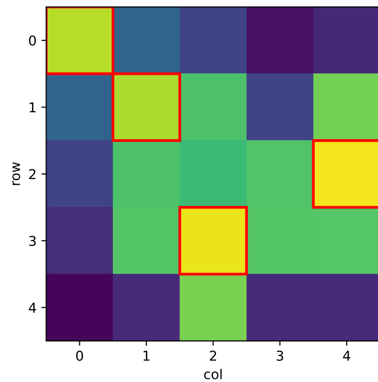
\alpha = 0.8, \lambda = 0.5
