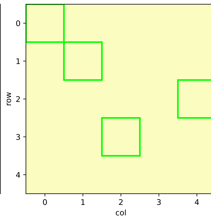
\alpha = 0.8, \lambda = 5.0
