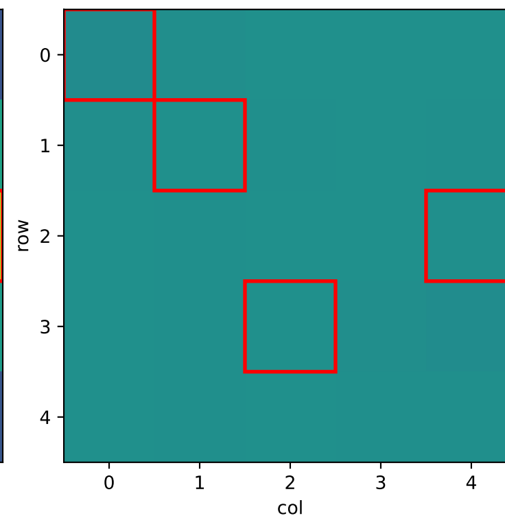
\alpha = 0.8, \lambda = 5.0
