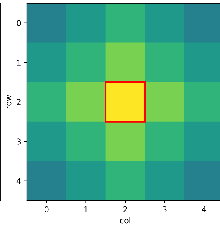
\alpha = 0.8, \lambda = 5.0
