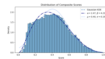
Figure 4. Score Distribution
