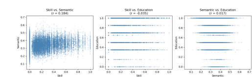
Figure 5. Scoring Correlates
