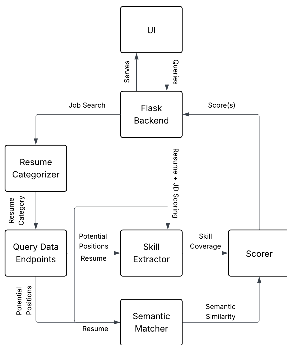
System Architecure
