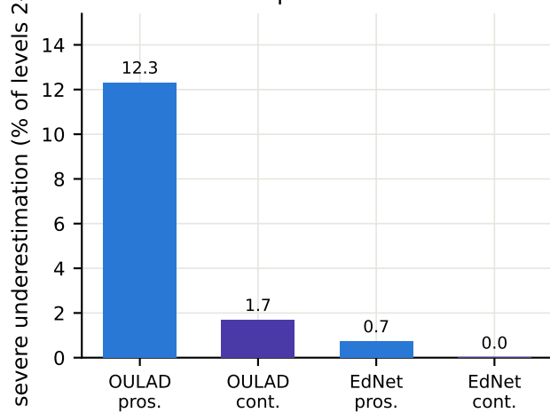
Severe cases predicted as low risk
