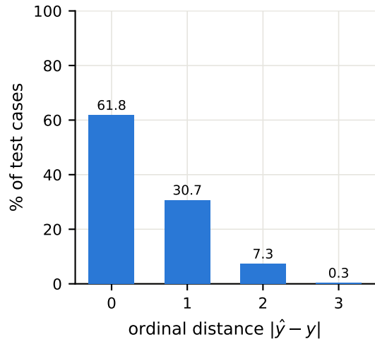
OULAD — XGBoost
