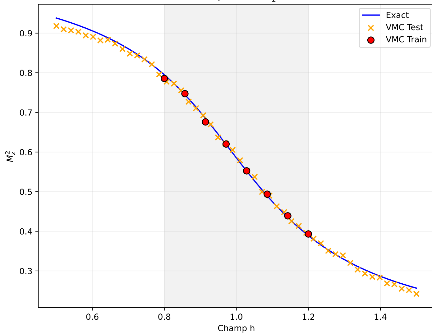
Comparaison M_z^2
