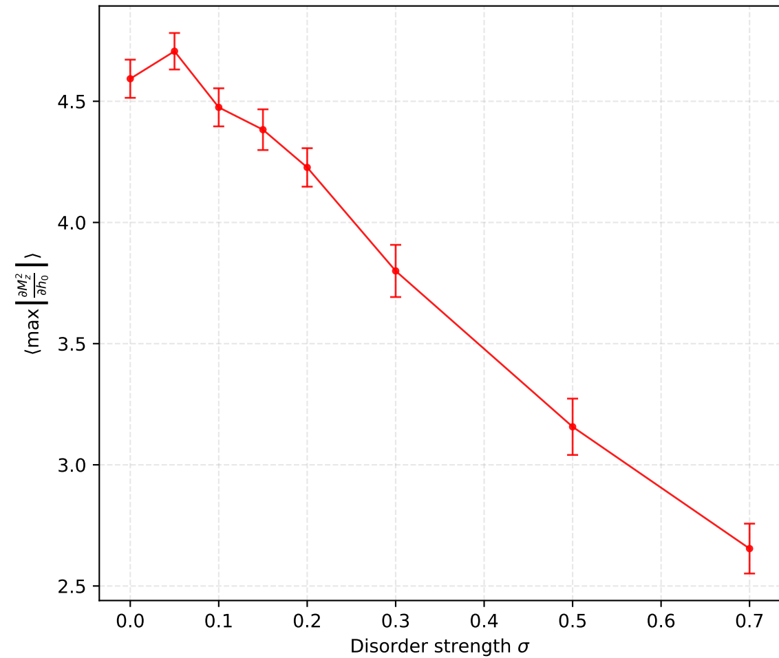
Mean of the Max Derivatives (Microscopic)
