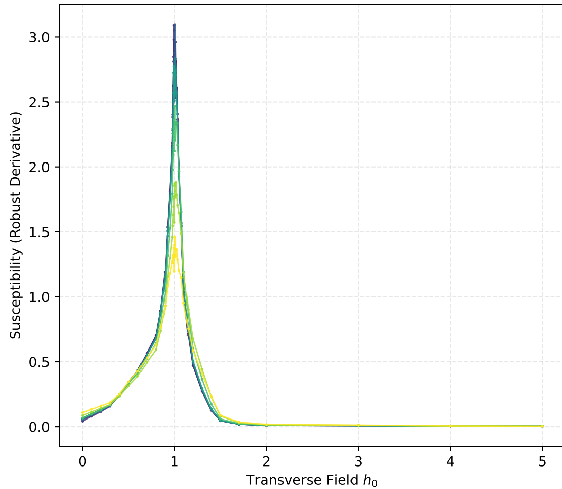
Derivative of Mean M_z^2 (span=3)
