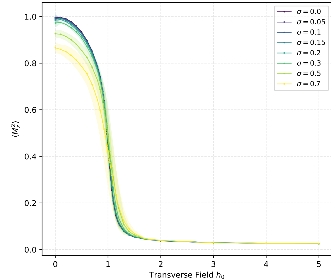
Mean Squared Magnetization
