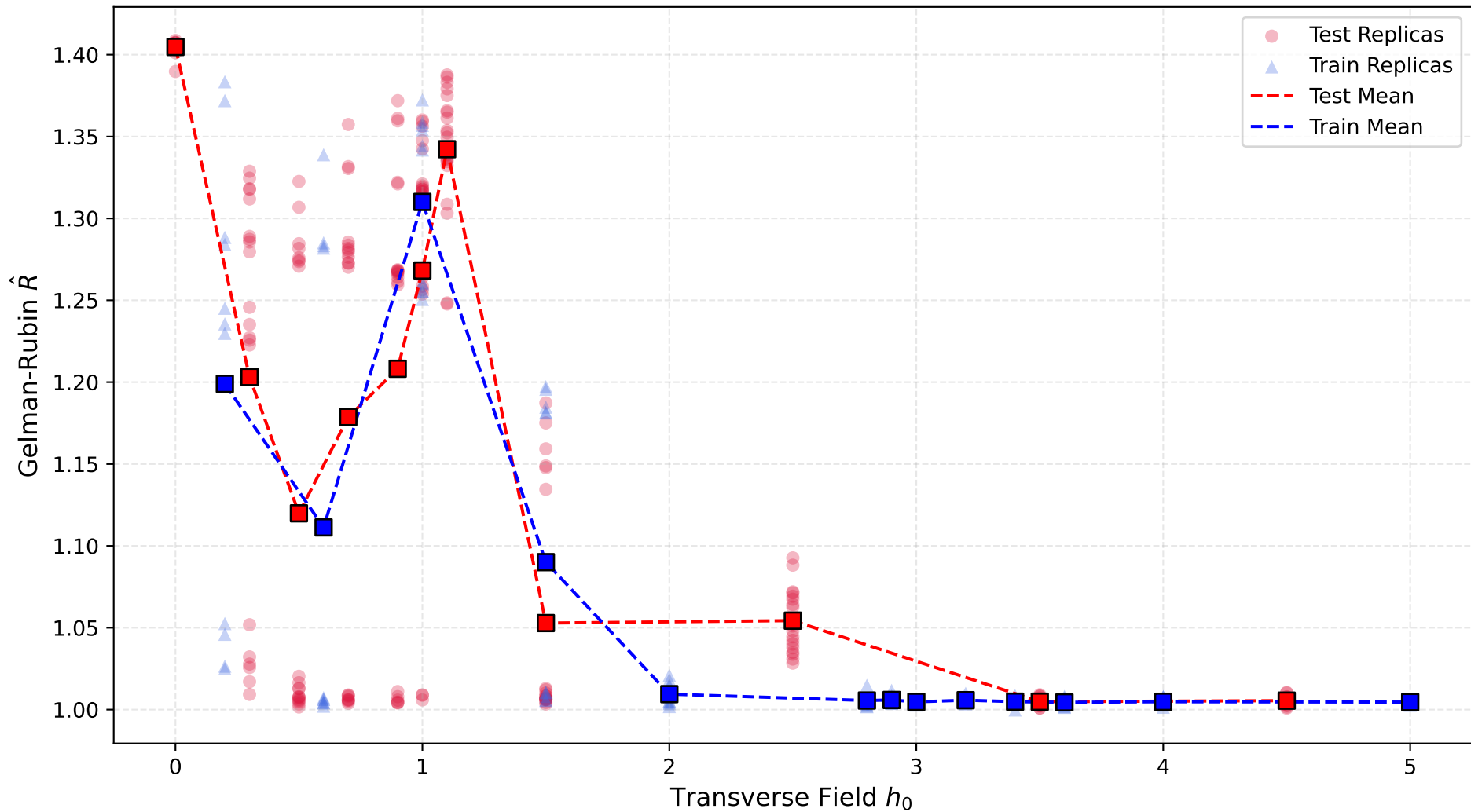
Convergence Diagnostics ( \hat{R} ): Train vs Test (Grid=10x10)
