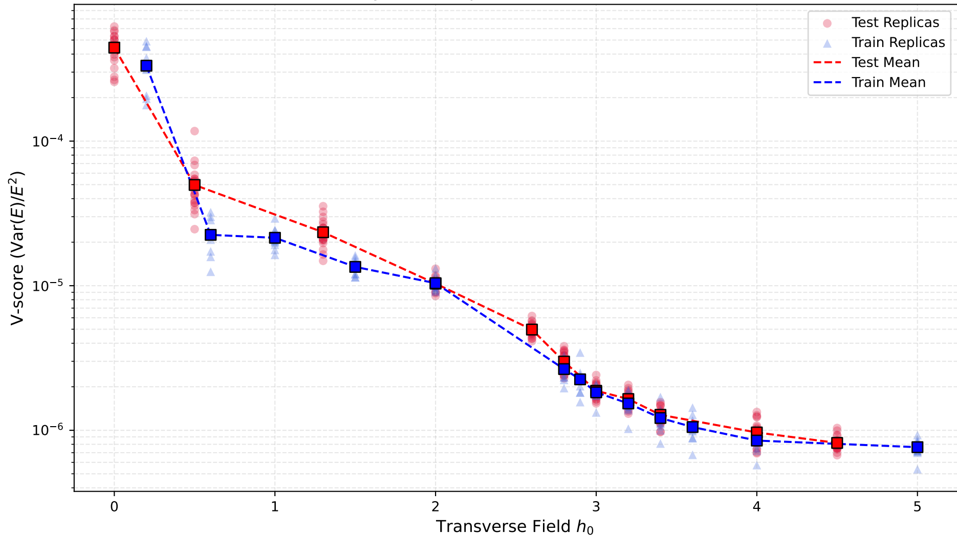
Accuracy Landscape: Train vs Test (Grid=4x4)
