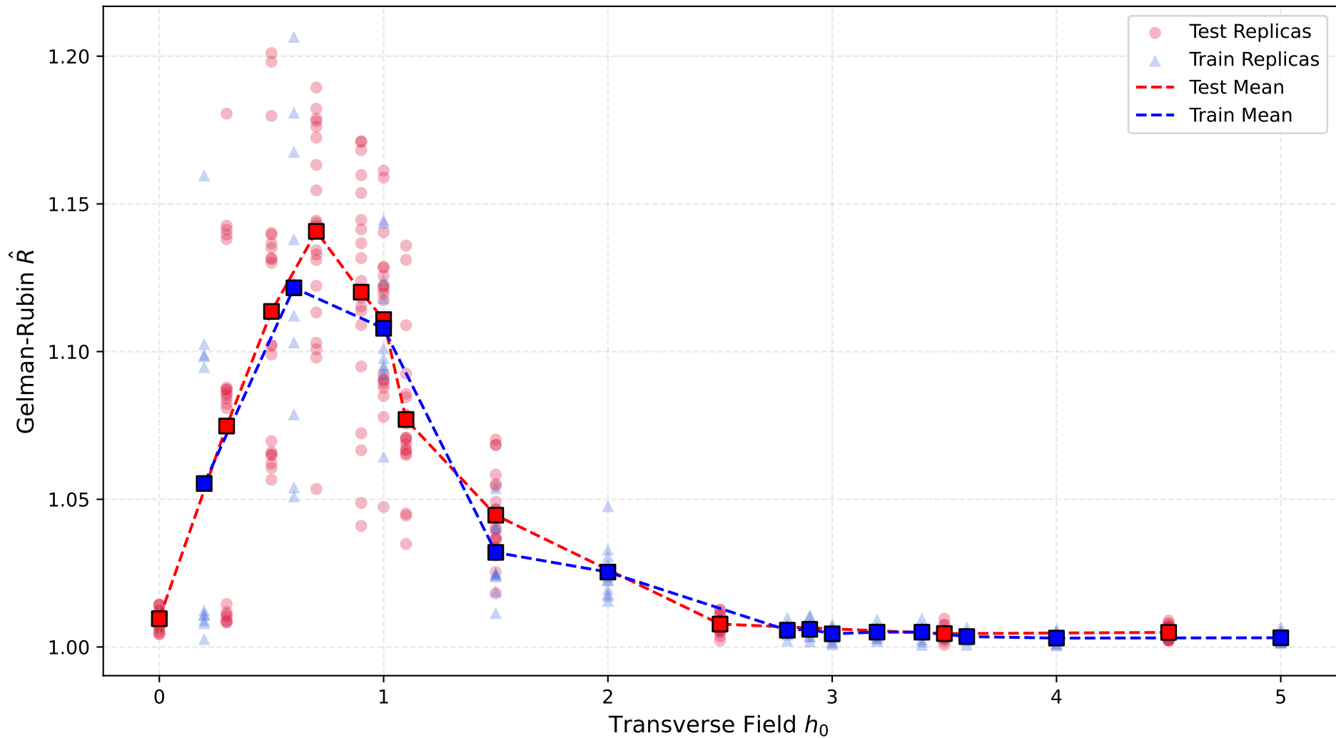
Convergence Diagnostics ( \hat{R} ): Train vs Test (Grid=8x8)
