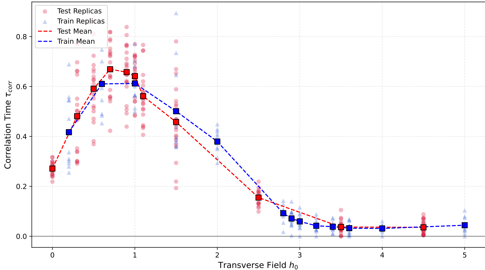
Sampling Efficiency ( \tau_{corr} ): Train vs Test (Grid=8x8)
