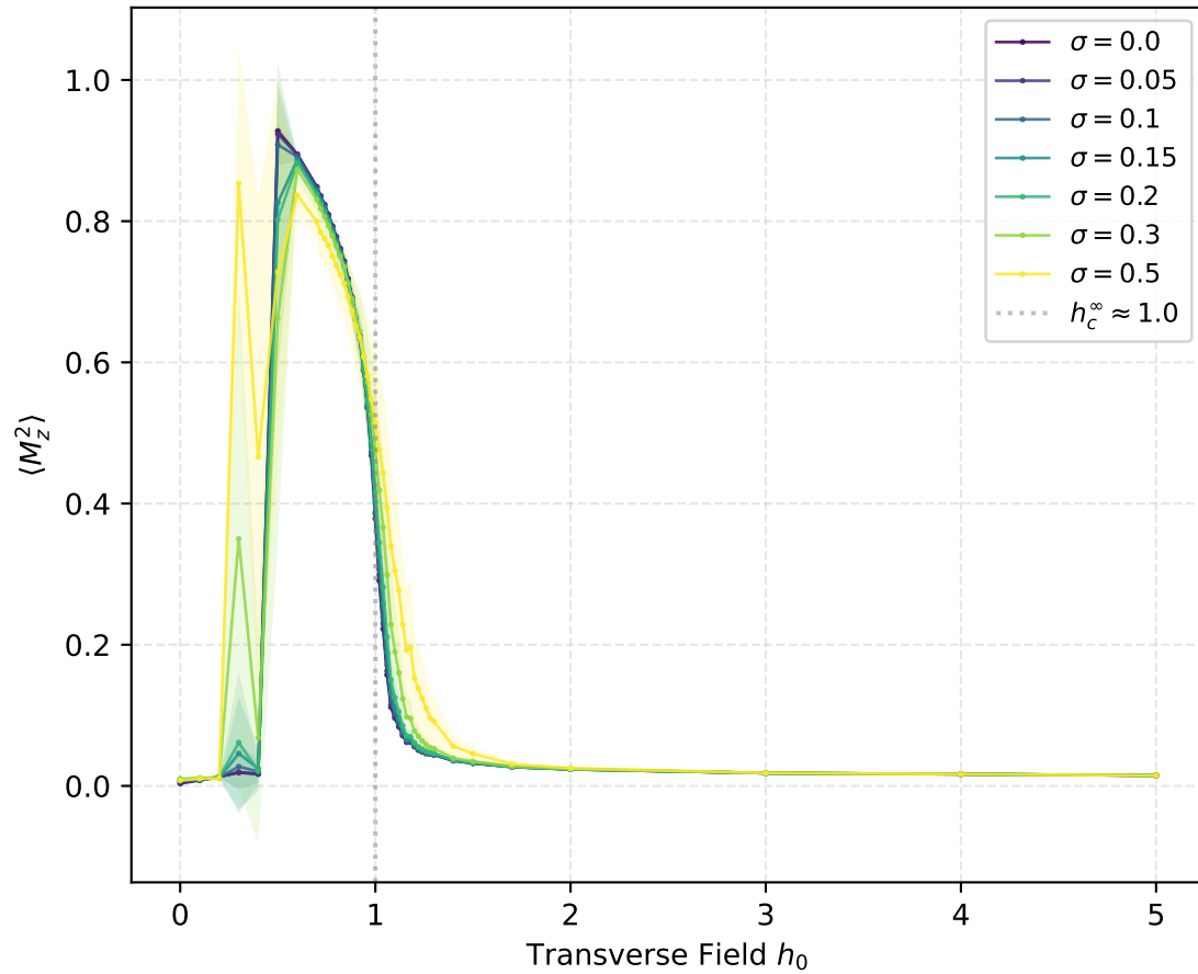
Mean Squared Magnetization — 1D L = 80 (80 spins)
