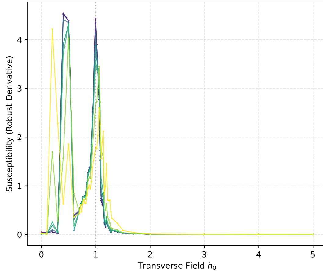
Derivative of Mean M_z^2 (span=1)
